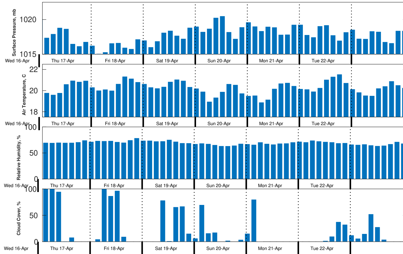
Met Forecast for Gyre from 16-Apr-2025 23:00:00 to 23-Apr-2025 23:00:00
