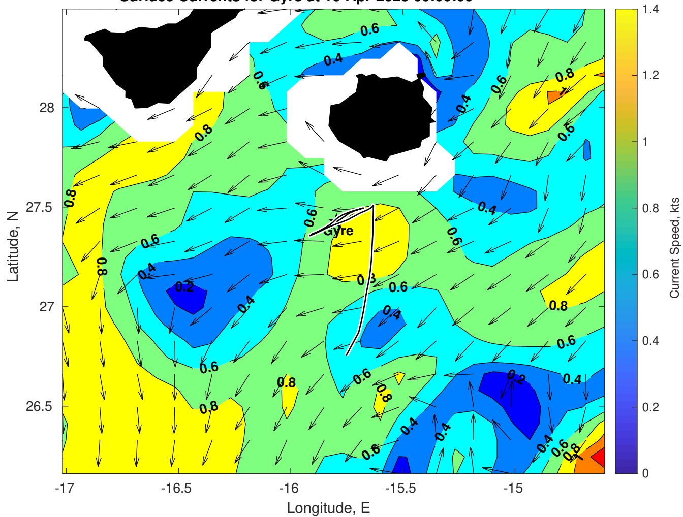
Surface Currents for Gyre at 16-Apr-2025 00:00:00
