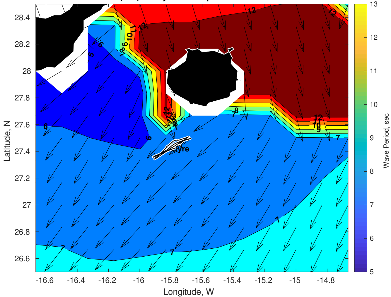
Wave Period (sec) for Gyre at 17-Apr-2025 09:00:00
