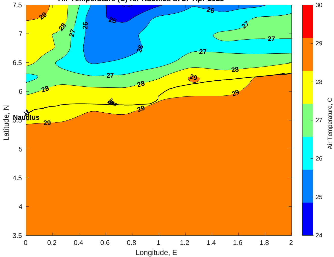
Air Temperature (C) for Nautilus at 17-Apr-2025
