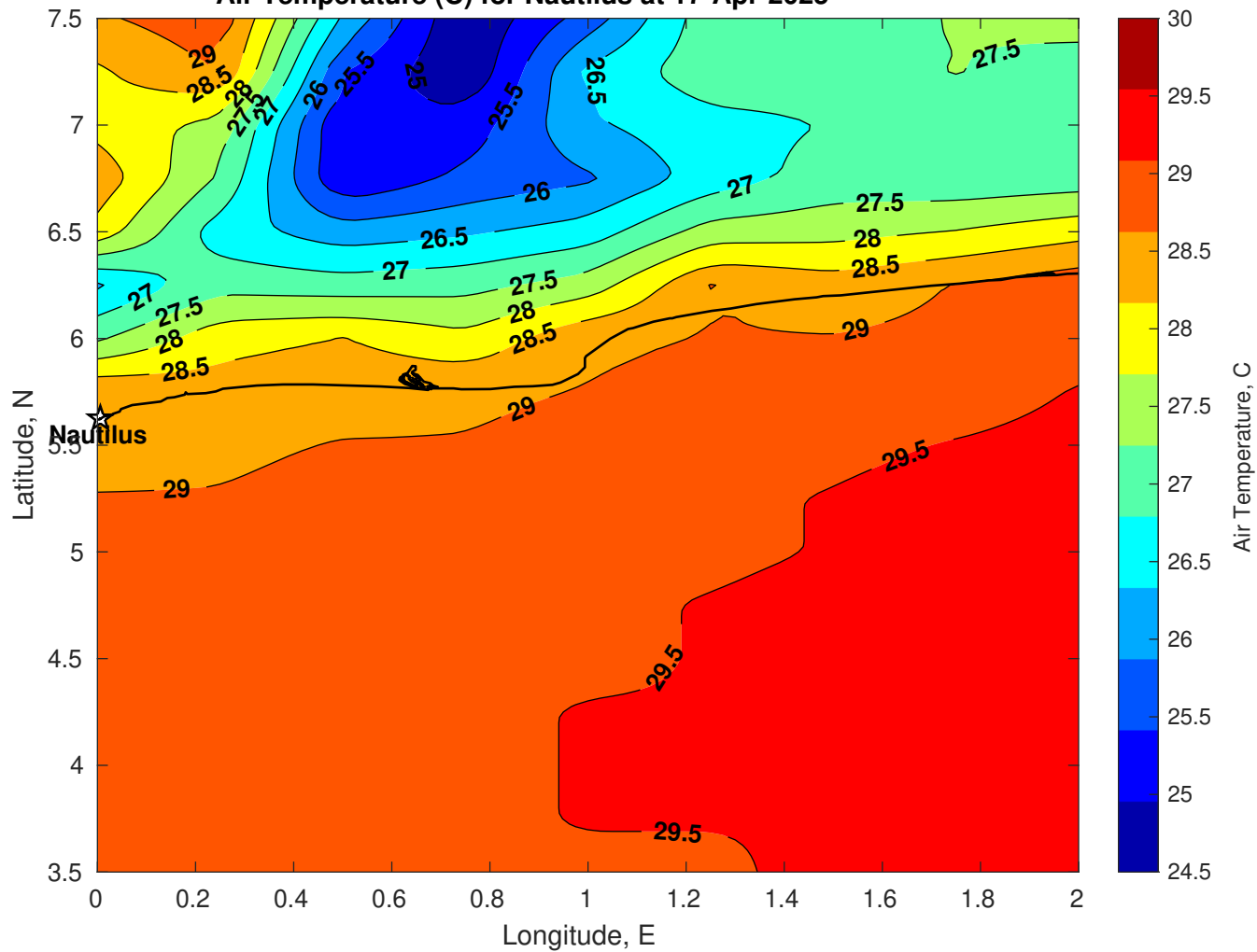
Air Temperature (C) for Nautilus at 17-Apr-2025
