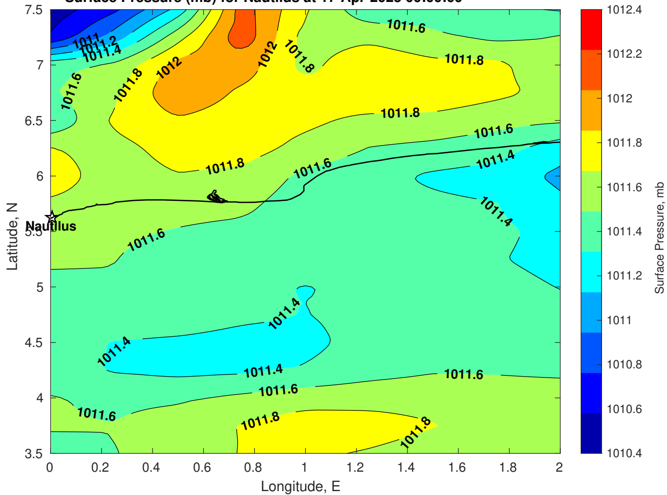
Surface Pressure (mb) for Nautilus at 17-Apr-2025 00:00:00
