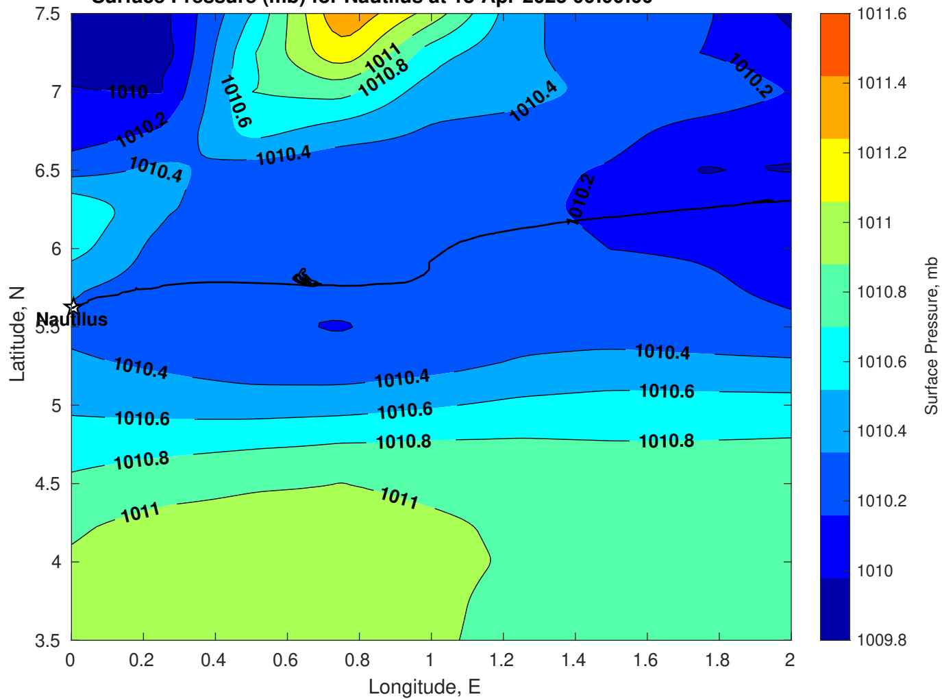
Surface Pressure (mb) for Nautilus at 18-Apr-2025 00:00:00
