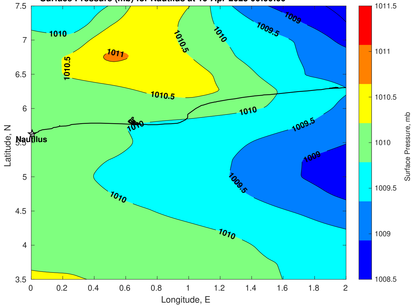
Surface Pressure (mb) for Nautilus at 19-Apr-2025 00:00:00
