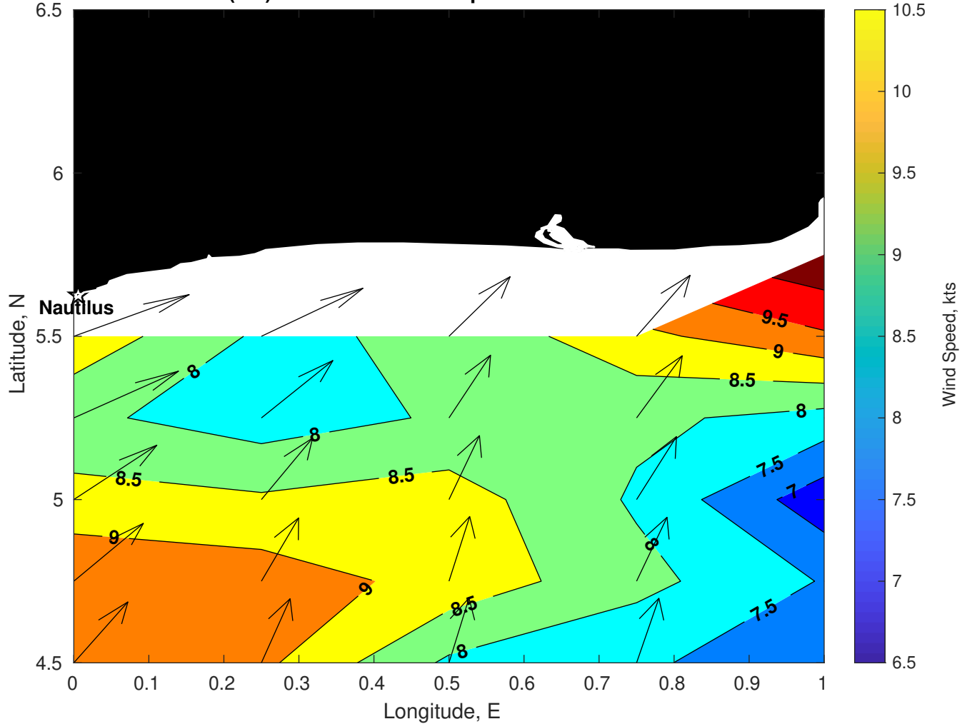
Winds (kts) for Nautilus at 17-Apr-2025 09:00:00
