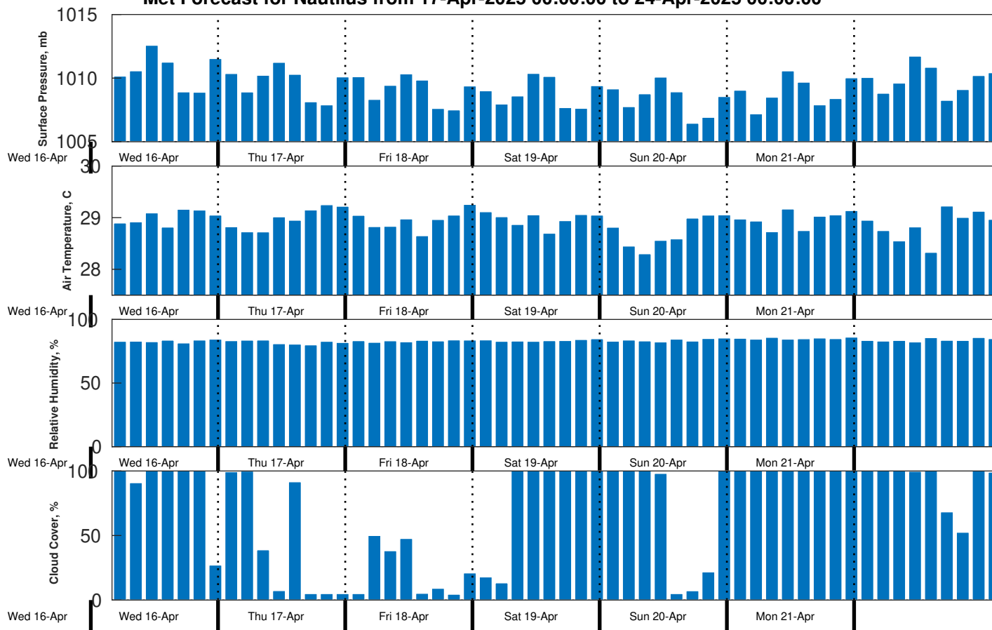
Met Forecast for Nautilus from 17-Apr-2025 00:00:00 to 24-Apr-2025 00:00:00
