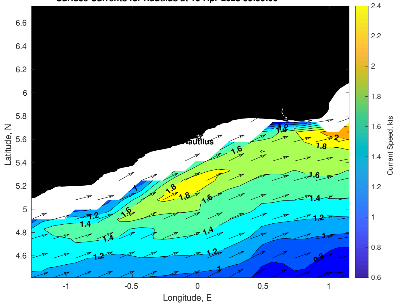
Surface Currents for Nautilus at 16-Apr-2025 00:00:00
