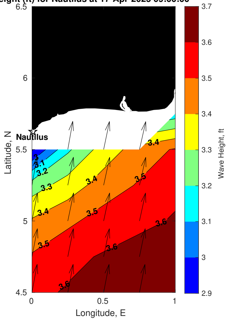
Wave Height (ft) for Nautilus at 17-Apr-2025 09:00:00
