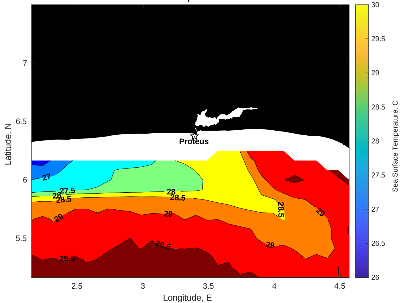
SST for Proteus at 16-Apr-2025 00:00:00
