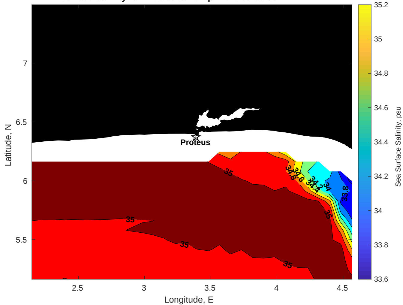
Surface Salinity for Proteus at 16-Apr-2025 00:00:00
