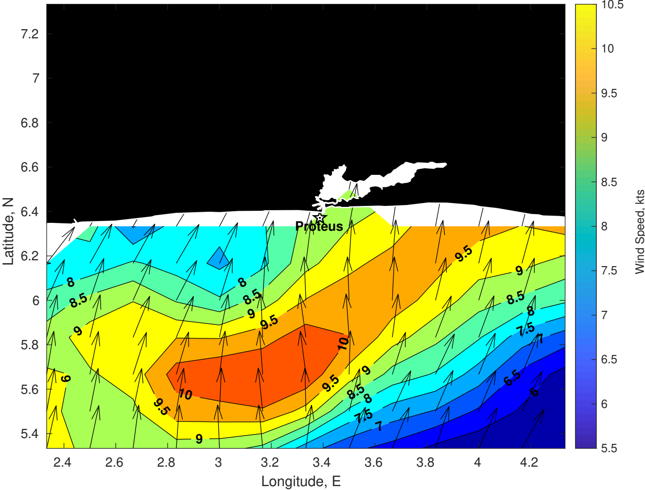
Winds (kts) for Proteus at 17-Apr-2025 09:00:00
