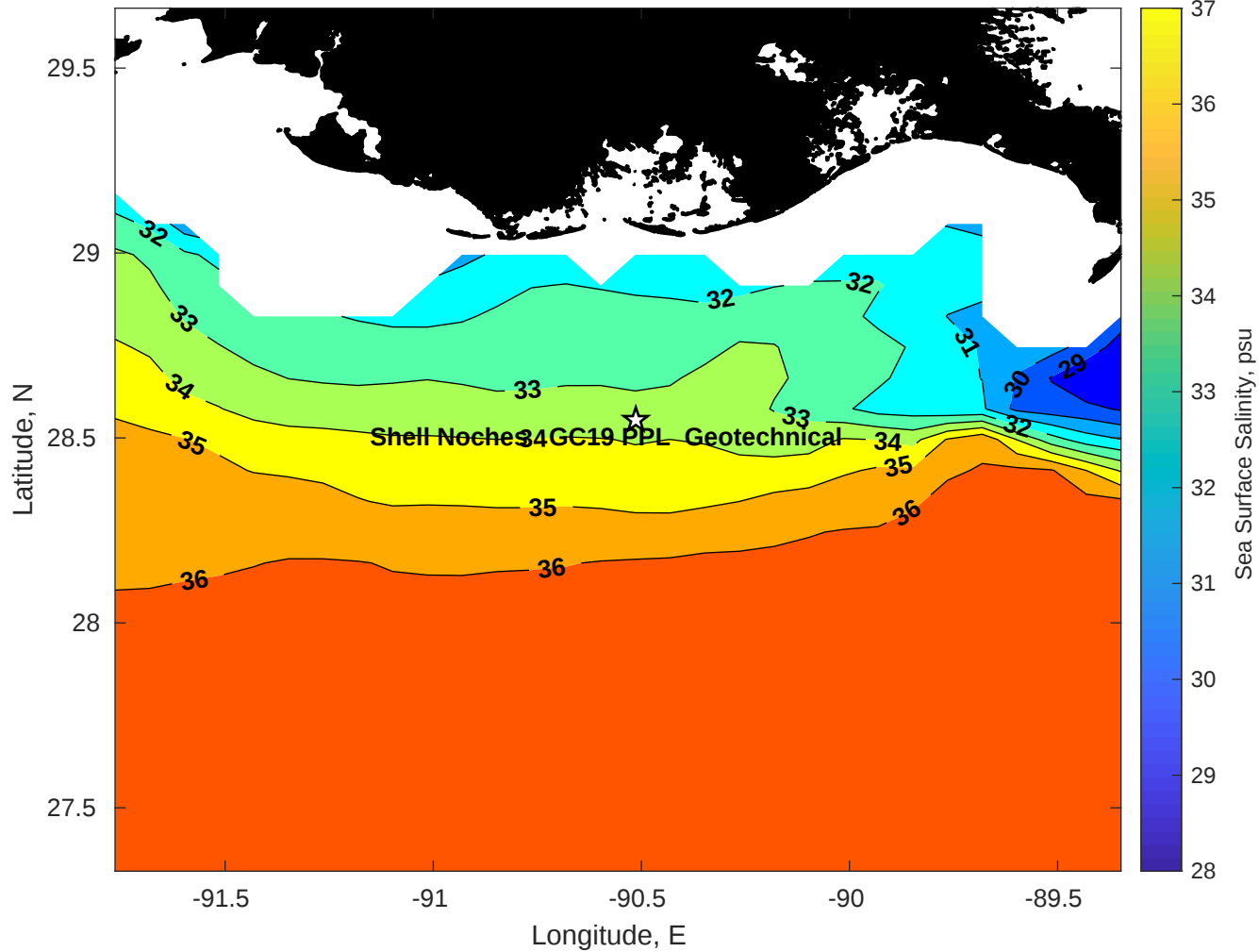
Surface Salinity for Shell Noches GC19 PPL Geotechnical at 16-Apr-2025 00:00:00
