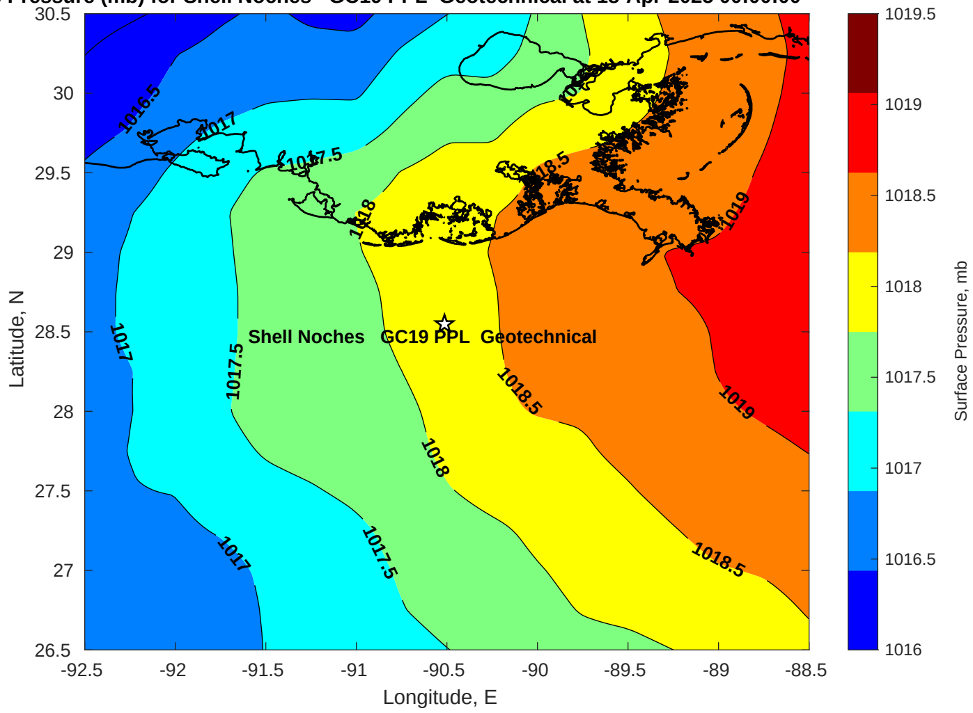
Surface Pressure (mb) for Shell Noches GC19 PPL Geotechnical at 18-Apr-2025 00:00:00
