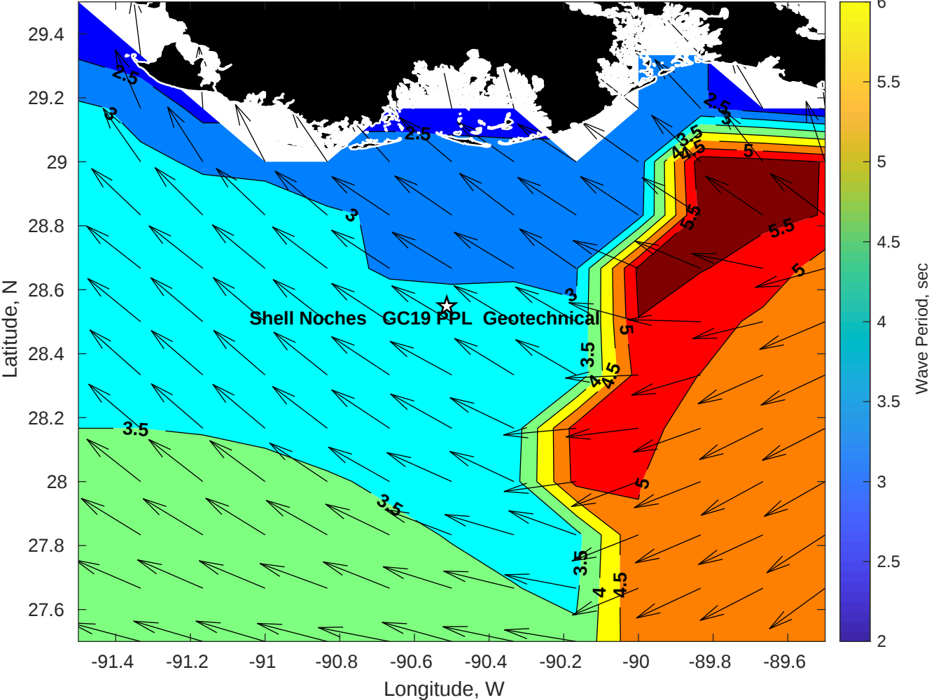
Wave Period (sec) for Shell Noches GC19 PPL Geotechnical at 17-Apr-2025 09:00:00
