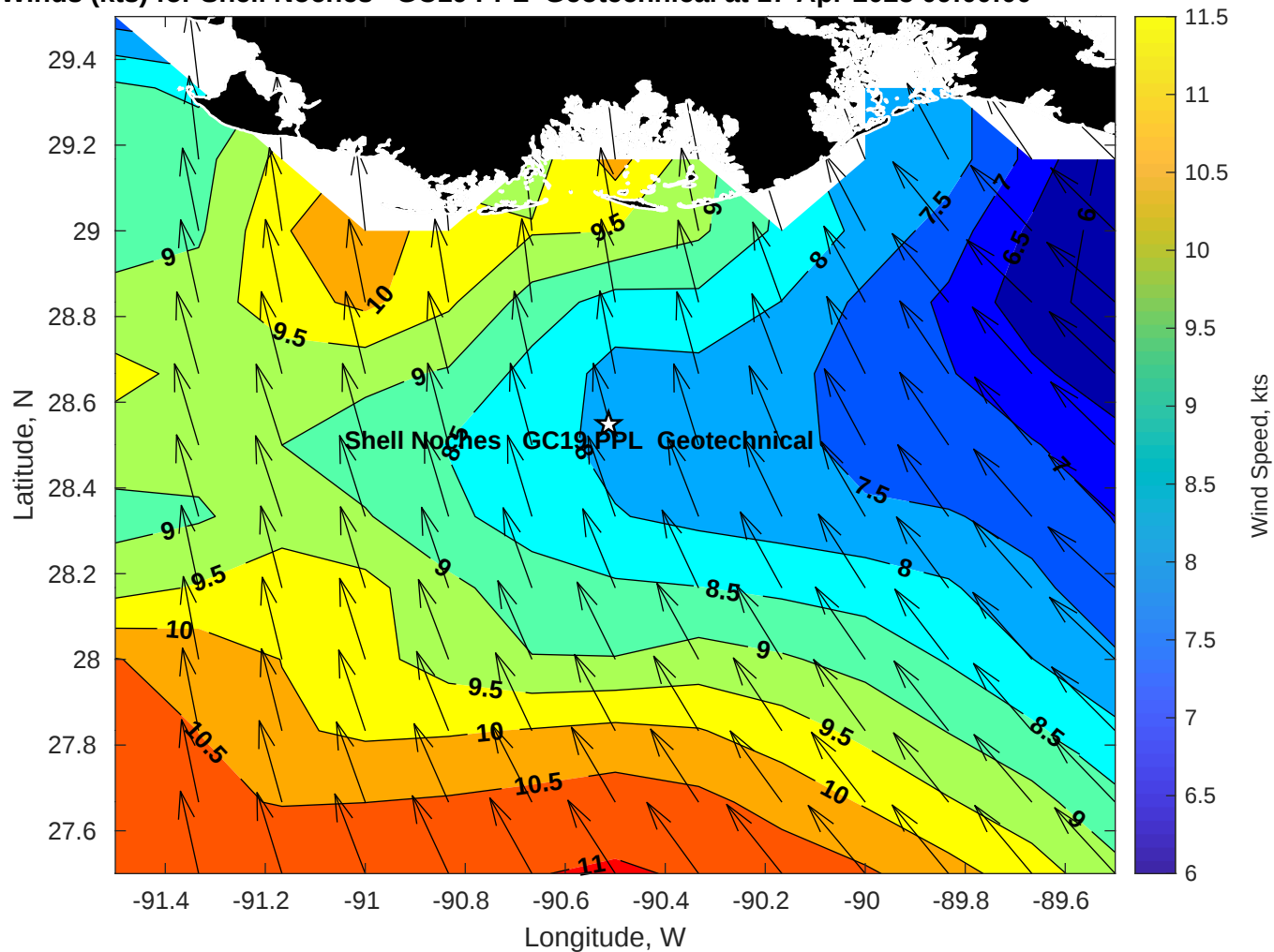
Winds (kts) for Shell Noches GC19 PPL Geotechnical at 17-Apr-2025 09:00:00
