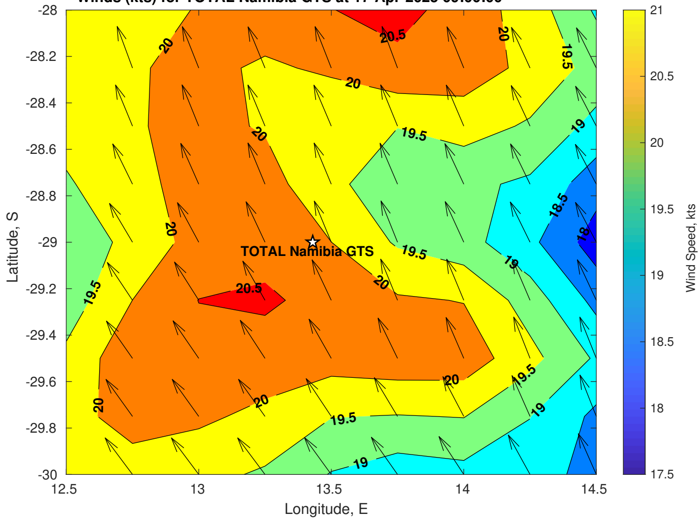
Winds (kts) for TOTAL Namibia GTS at 17-Apr-2025 09:00:00
