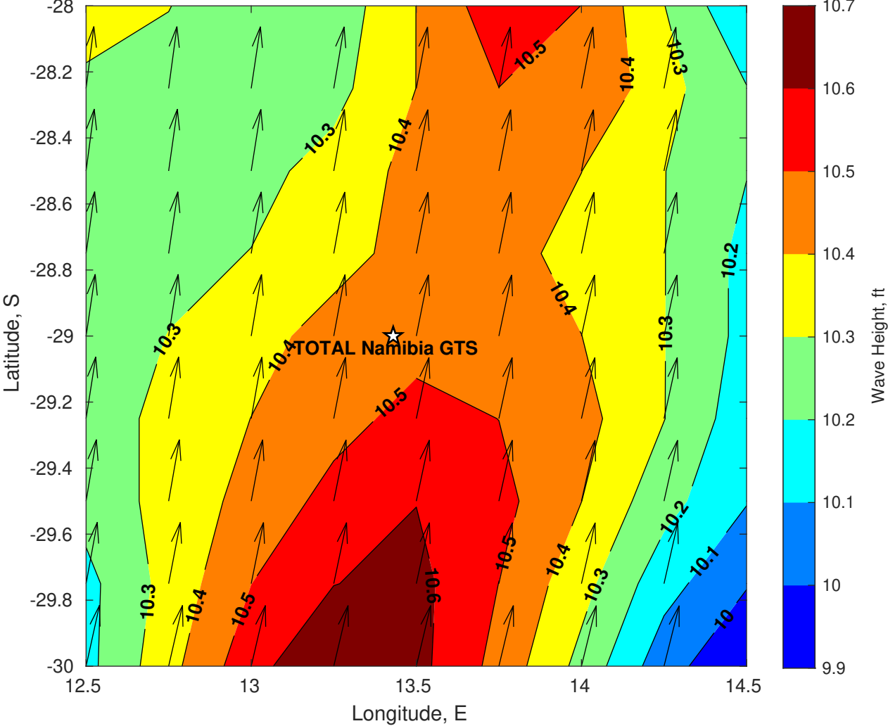
Wave Height (ft) for TOTAL Namibia GTS at 17-Apr-2025 09:00:00
