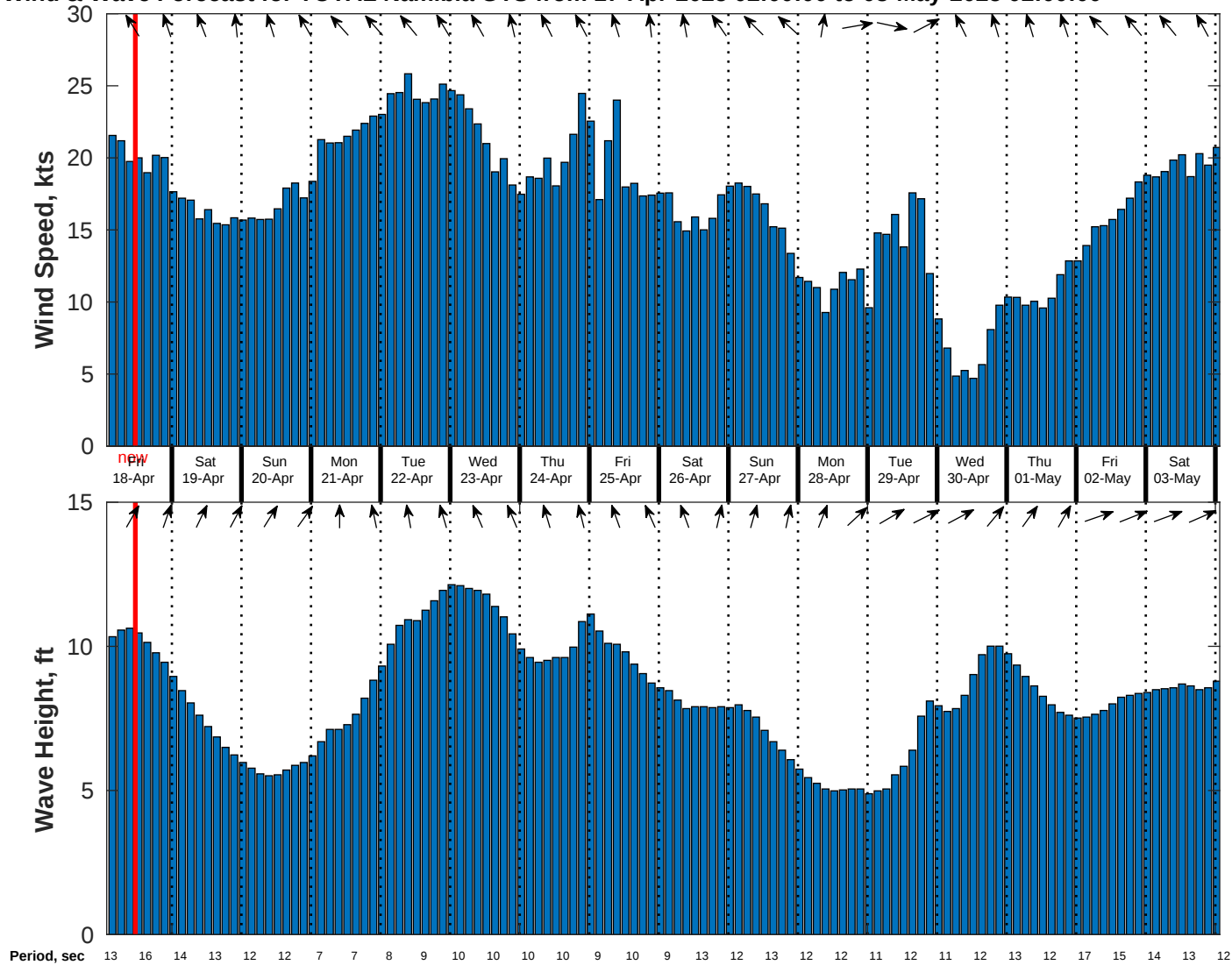
Wind & Wave Forecast for TOTAL Namibia GTS from 17-Apr-2025 02:00:00 to 03-May-2025 02:00:00
