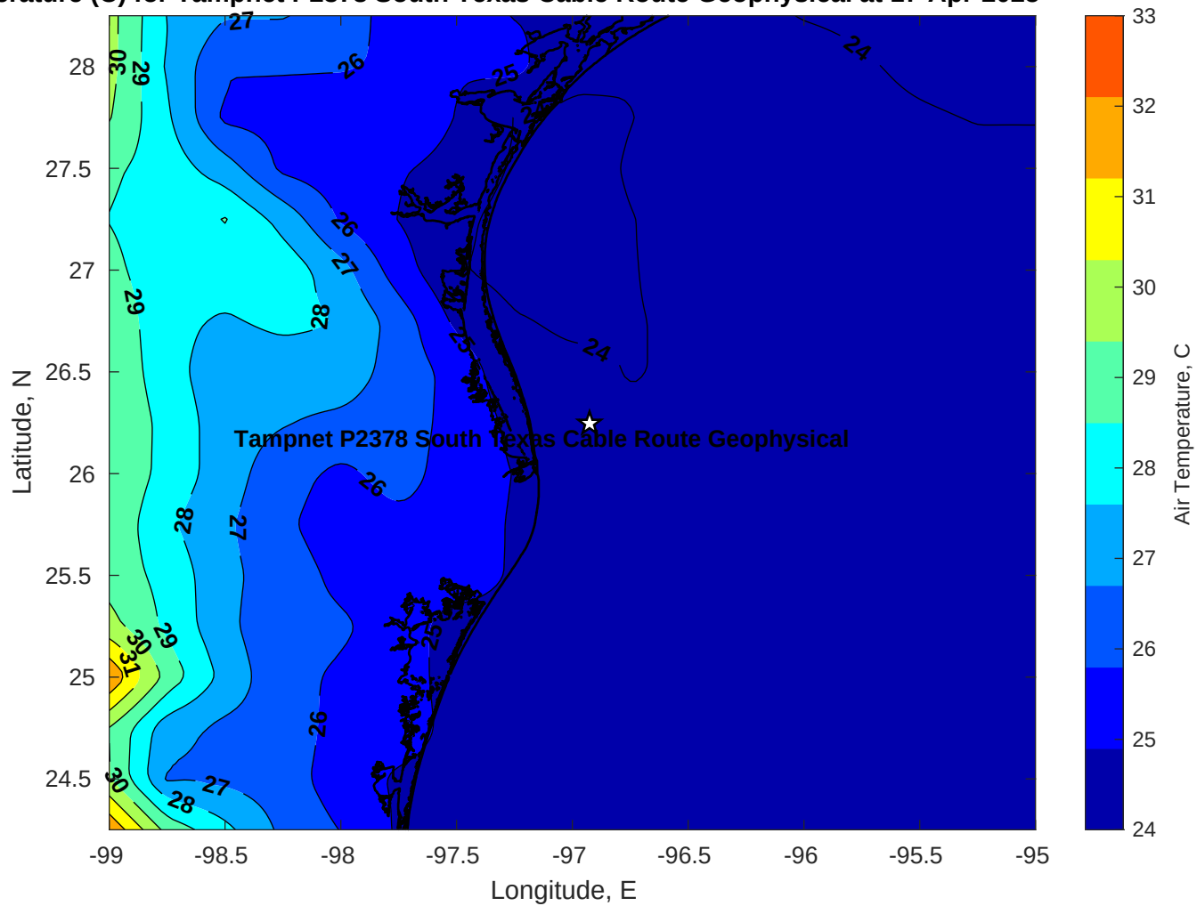
Air Temperature (C) for Tampnet P2378 South Texas Cable Route Geophysical at 17-Apr-2025
