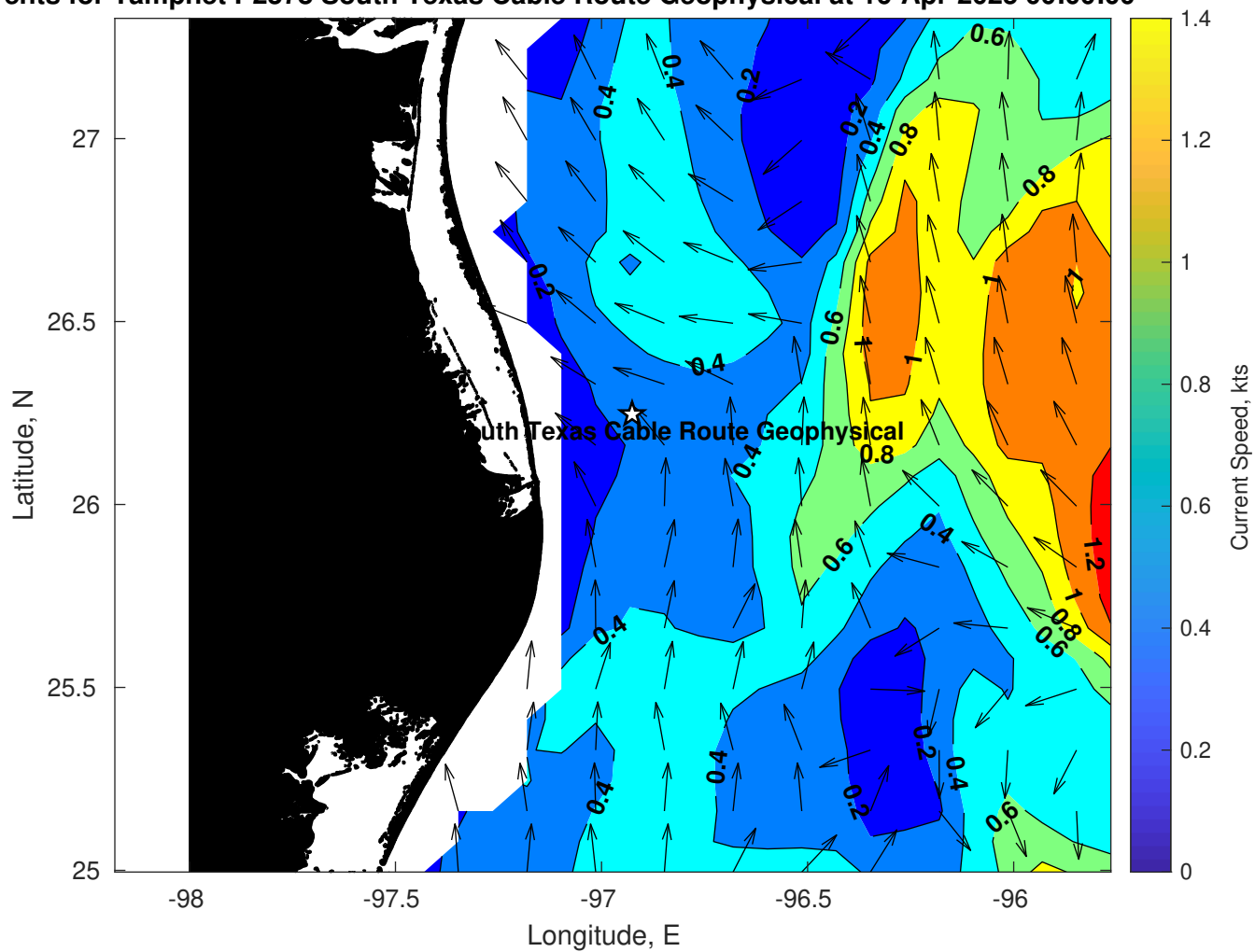
Surface Currents for Tampnet P2378 South Texas Cable Route Geophysical at 16-Apr-2025 00:00:00
