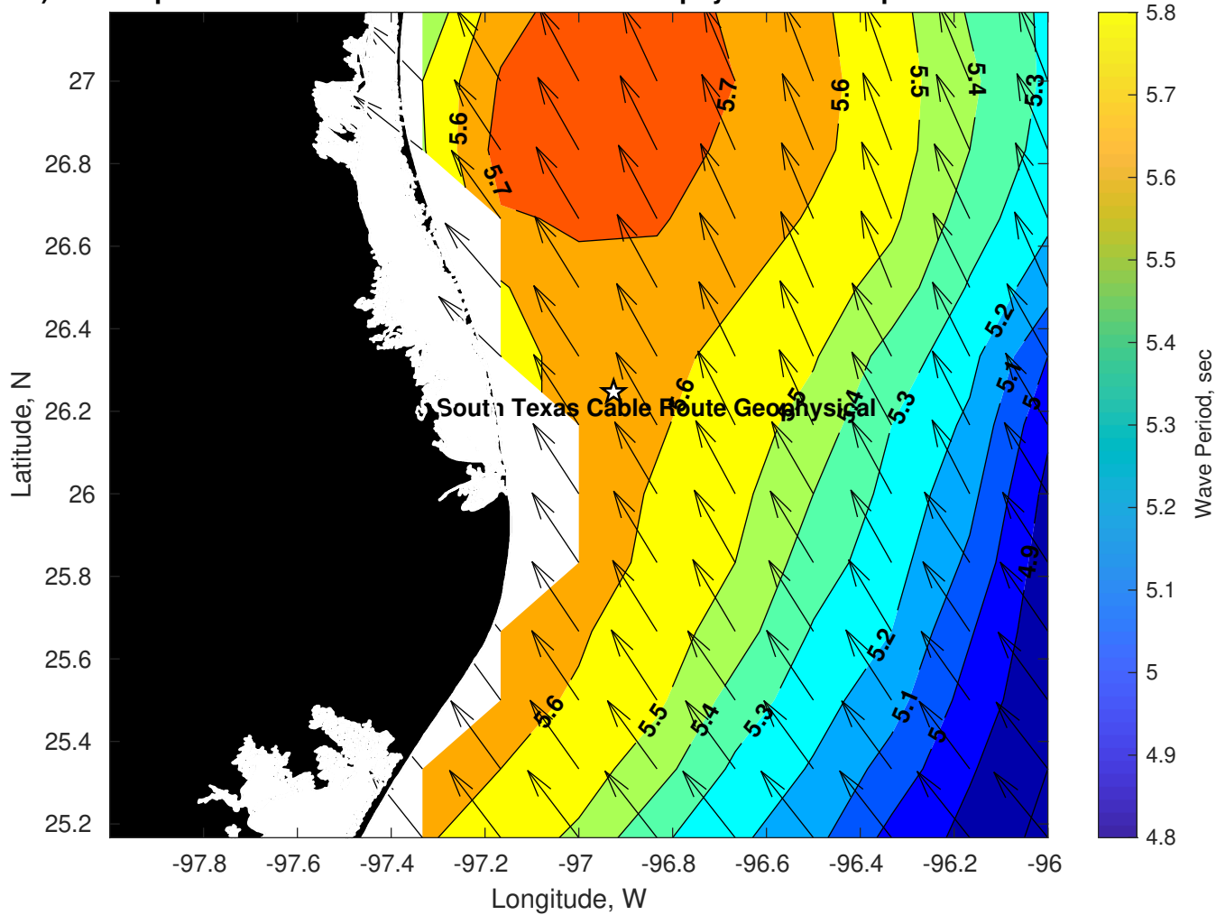
Period (sec) for Tampnet P2378 South Texas Cable Route Geophysical at 17-Apr-2025 09:00:00
