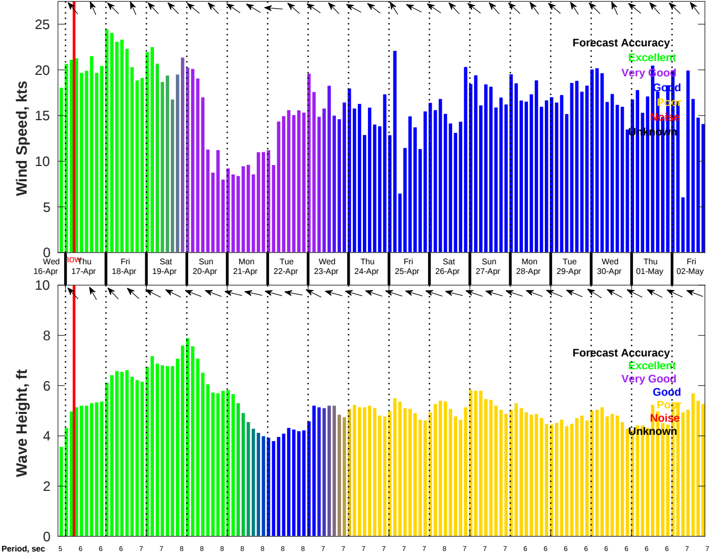
Wind & Wave Forecast for Tampnet P2378 South Texas Cable Route Geophysical from 16-Apr-2025 20:00:00 to 02-May-2025 20:00:00
