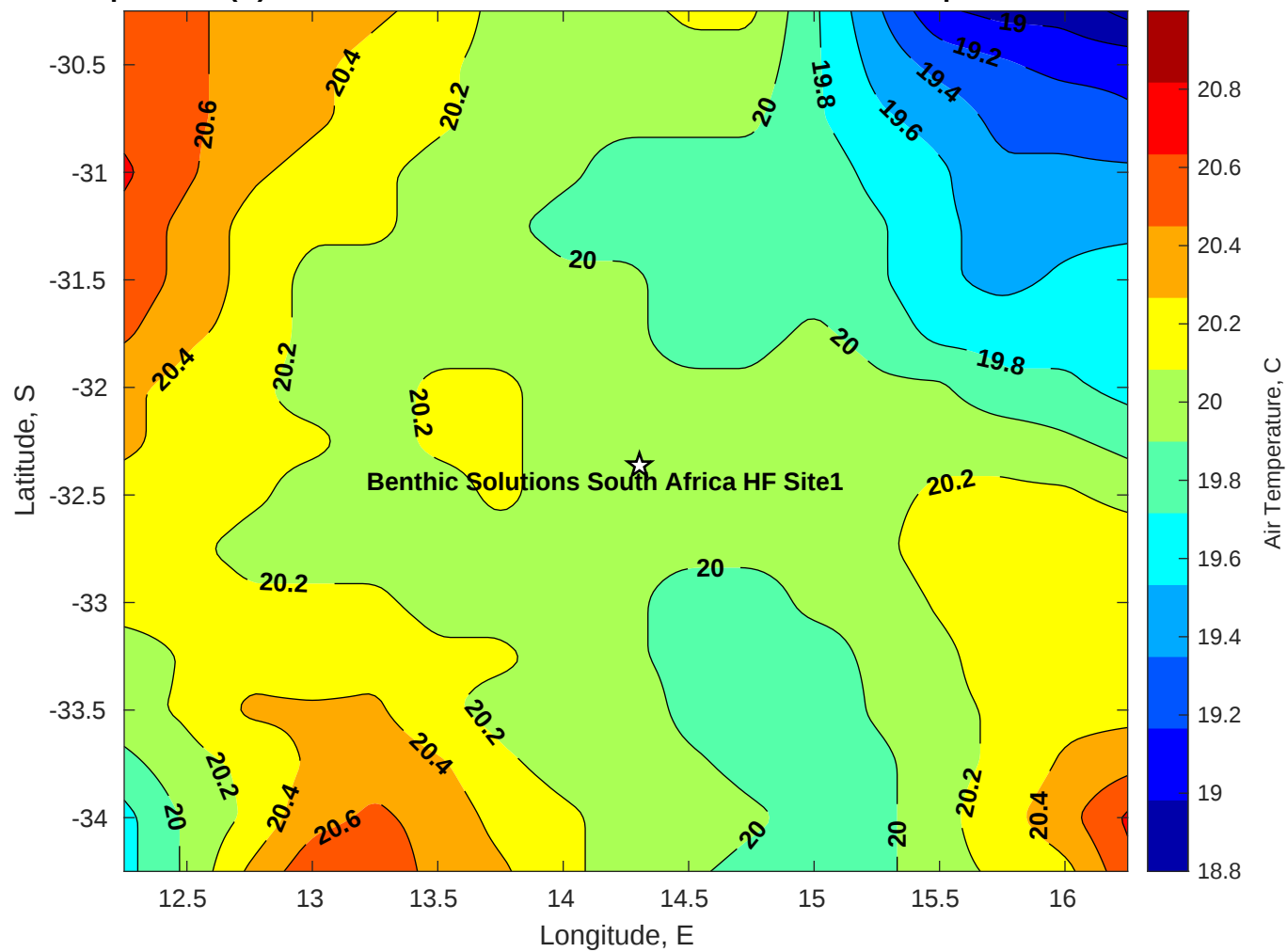
Air Temperature (C) for Benthic Solutions South Africa HF Site1 at 18-Apr-2025
