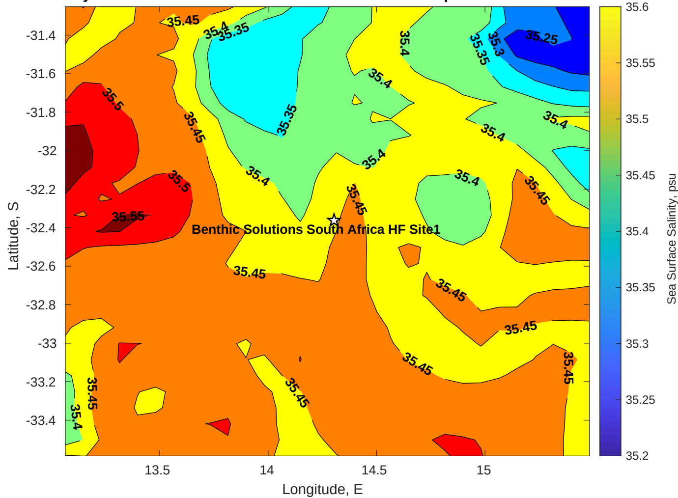
Surface Salinity for Benthic Solutions South Africa HF Site1 at 17-Apr-2025 00:00:00
