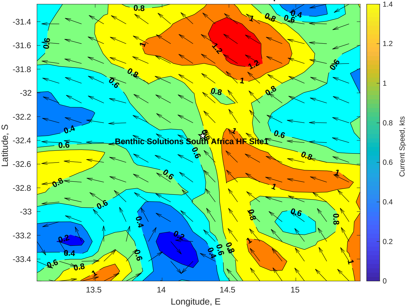
Surface Currents for Benthic Solutions South Africa HF Site1 at 17-Apr-2025 00:00:00
