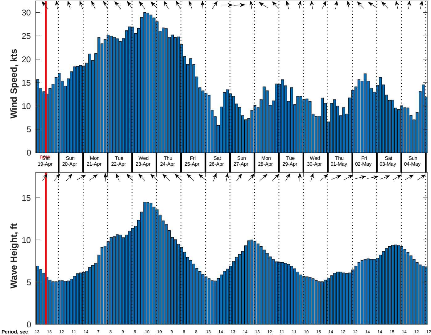
Wind & Wave Forecast for Benthic Solutions South Africa HF Site1 from 18-Apr-2025 02:00:00 to 04-May-2025 02:00:00
