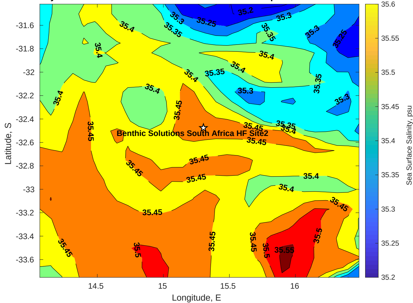
Surface Salinity for Benthic Solutions South Africa HF Site2 at 17-Apr-2025 00:00:00
