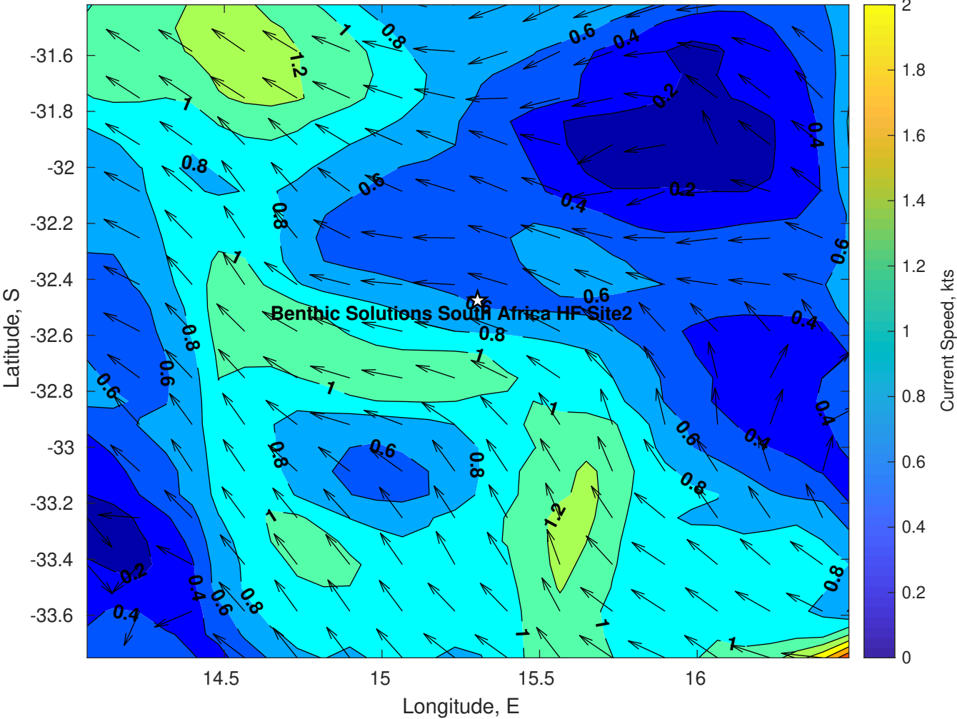
Surface Currents for Benthic Solutions South Africa HF Site2 at 17-Apr-2025 00:00:00
