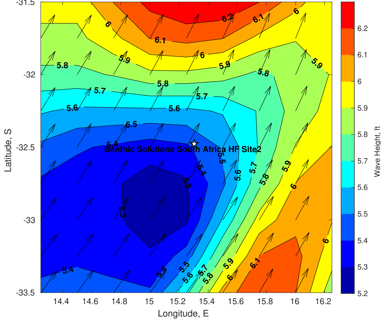
Wave Height (ft) for Benthic Solutions South Africa HF Site2 at 18-Apr-2025 09:00:00
