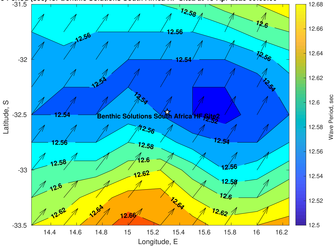
Wave Period (sec) for Benthic Solutions South Africa HF Site2 at 18-Apr-2025 09:00:00
