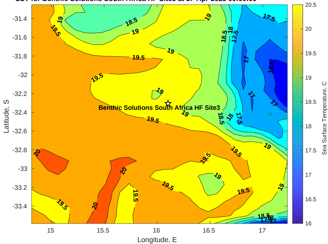
SST for Benthic Solutions South Africa HF Site3 at 17-Apr-2025 00:00:00
