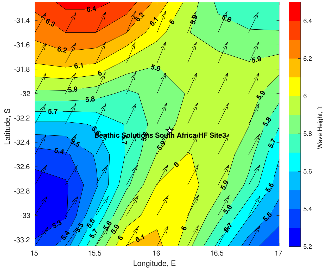
Wave Height (ft) for Benthic Solutions South Africa HF Site3 at 18-Apr-2025 09:00:00
