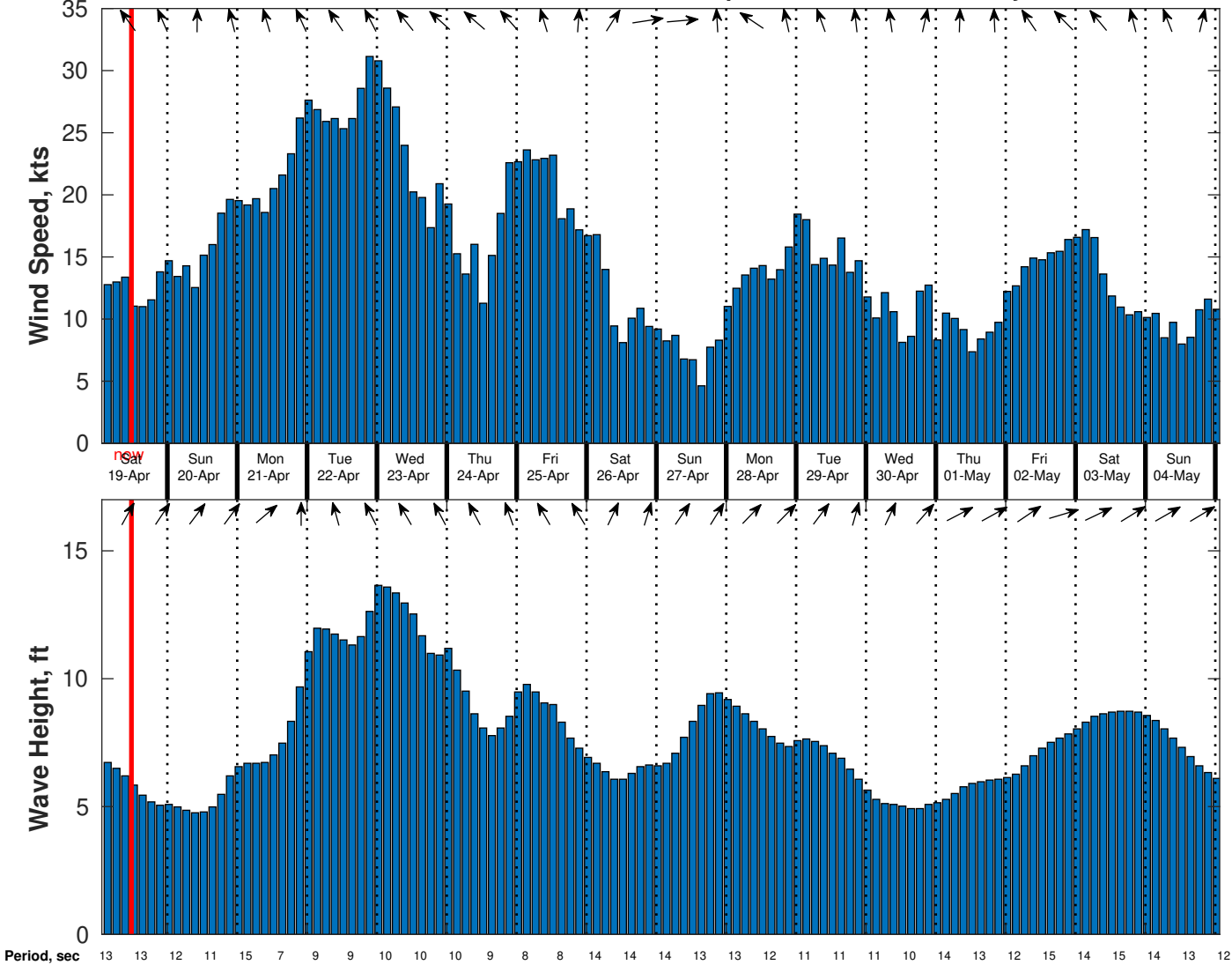
Wind & Wave Forecast for Benthic Solutions South Africa HF Site3 from 18-Apr-2025 02:00:00 to 04-May-2025 02:00:00
