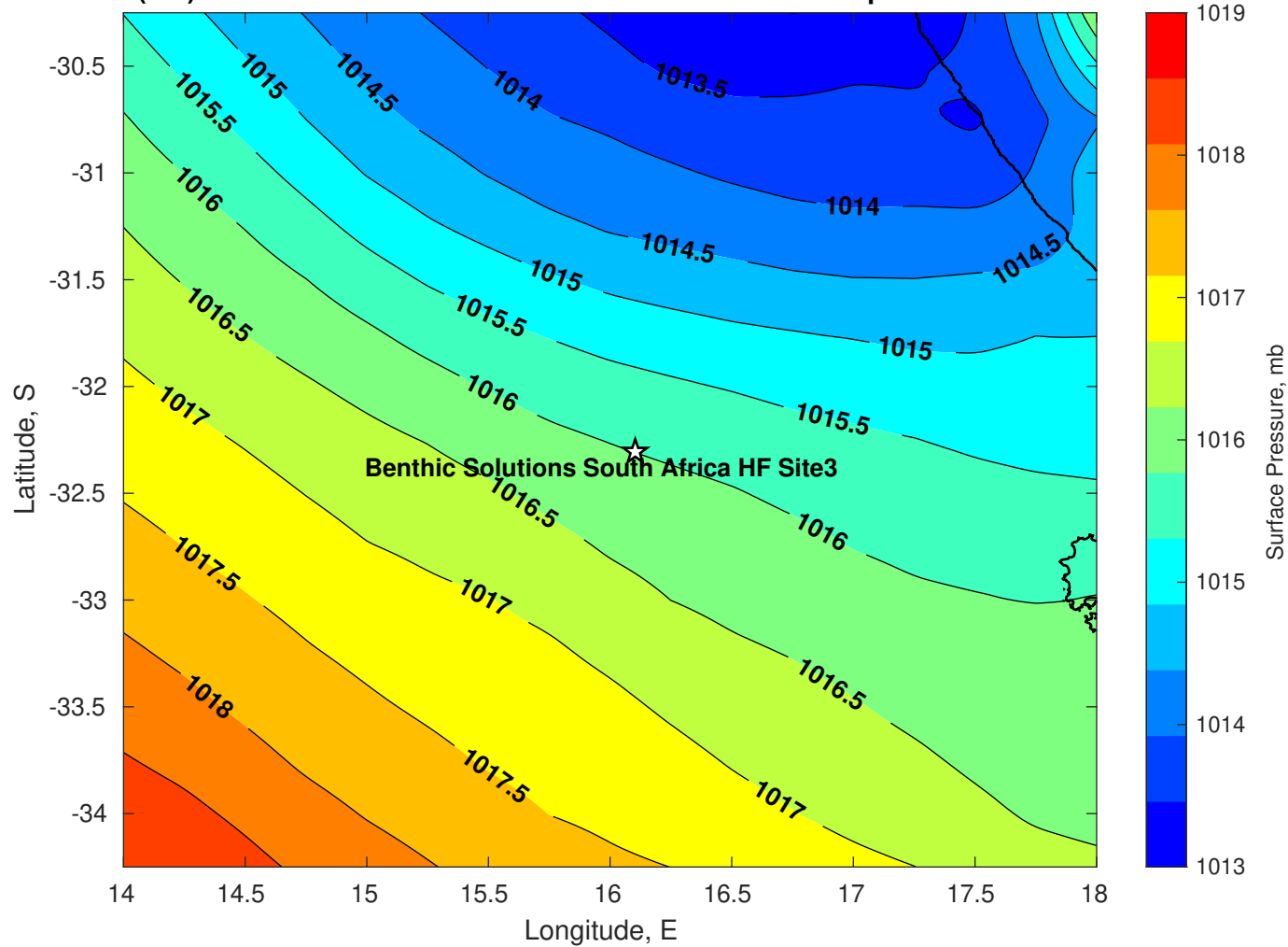
Surface Pressure (mb) for Benthic Solutions South Africa HF Site3 at 18-Apr-2025 00:00:00
