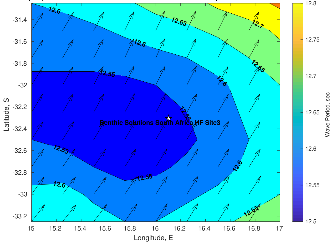
Wave Period (sec) for Benthic Solutions South Africa HF Site3 at 18-Apr-2025 09:00:00
