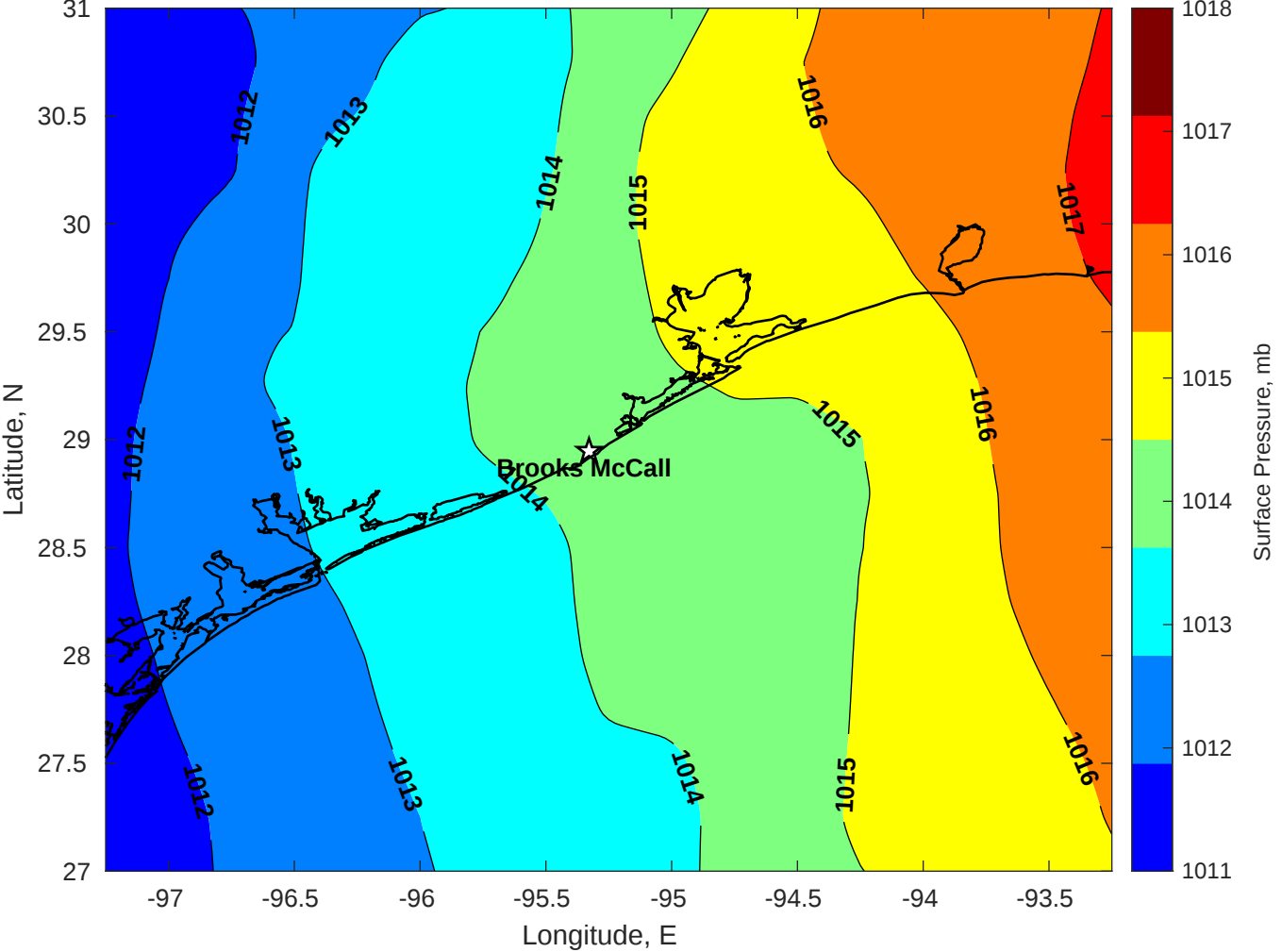
Surface Pressure (mb) for Brooks McCall at 20-Apr-2025 00:00:00
