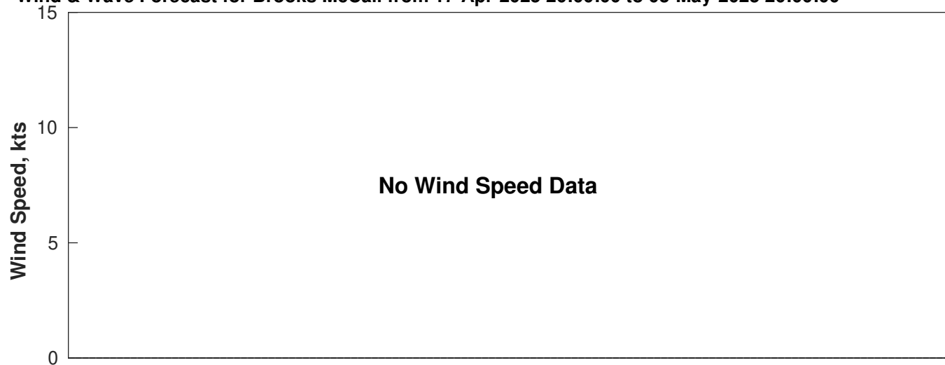
Wind & Wave Forecast for Brooks McCall from 17-Apr-2025 20:00:00 to 03-May-2025 20:00:00
