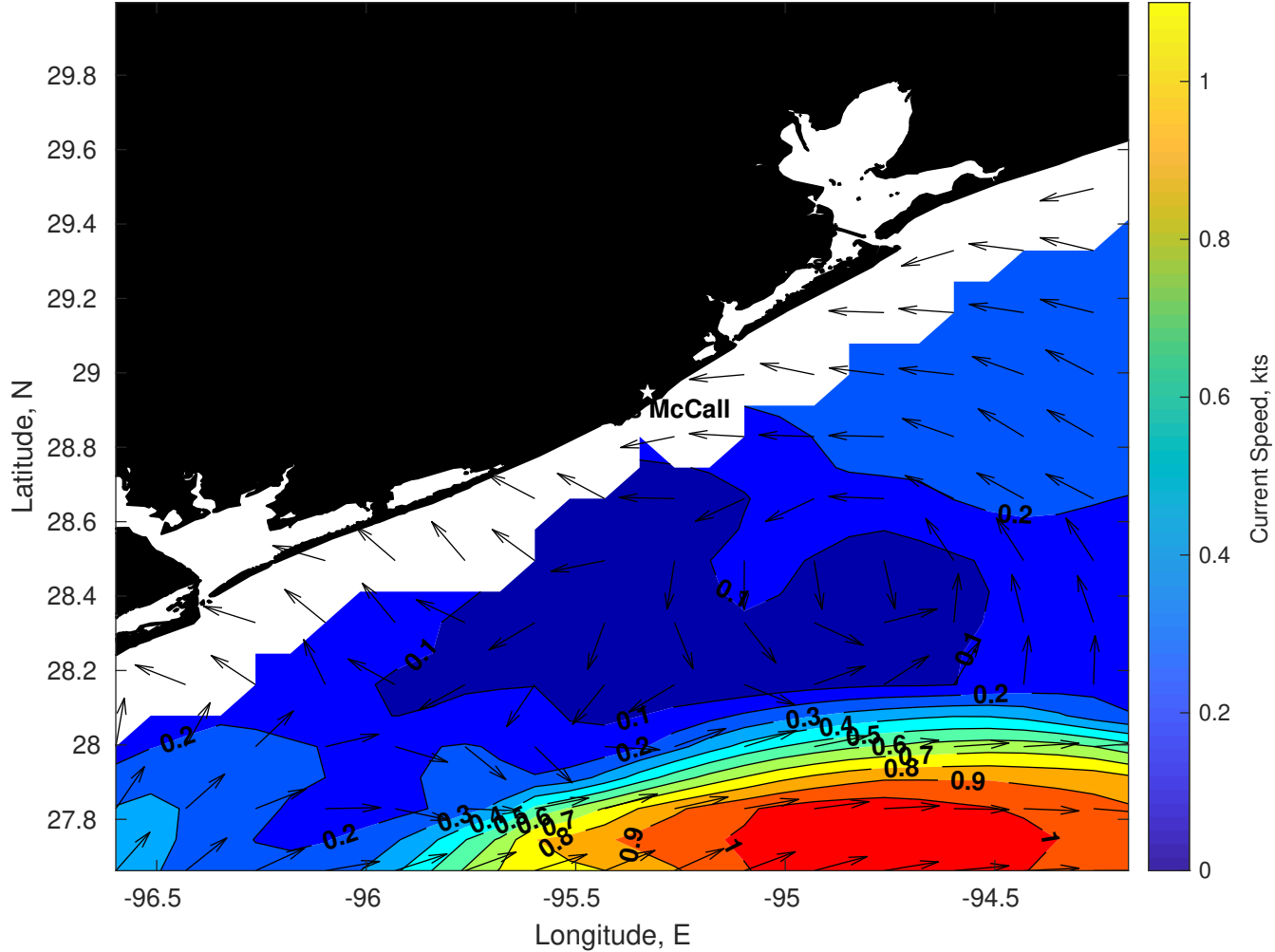
Surface Currents for Brooks McCall at 17-Apr-2025 00:00:00
