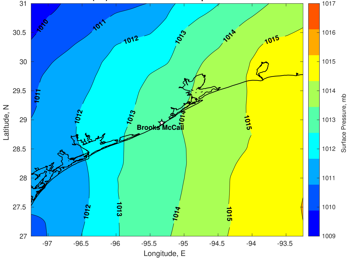
Surface Pressure (mb) for Brooks McCall at 18-Apr-2025 00:00:00
