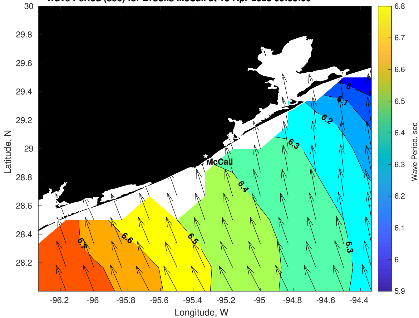
Wave Period (sec) for Brooks McCall at 18-Apr-2025 09:00:00
