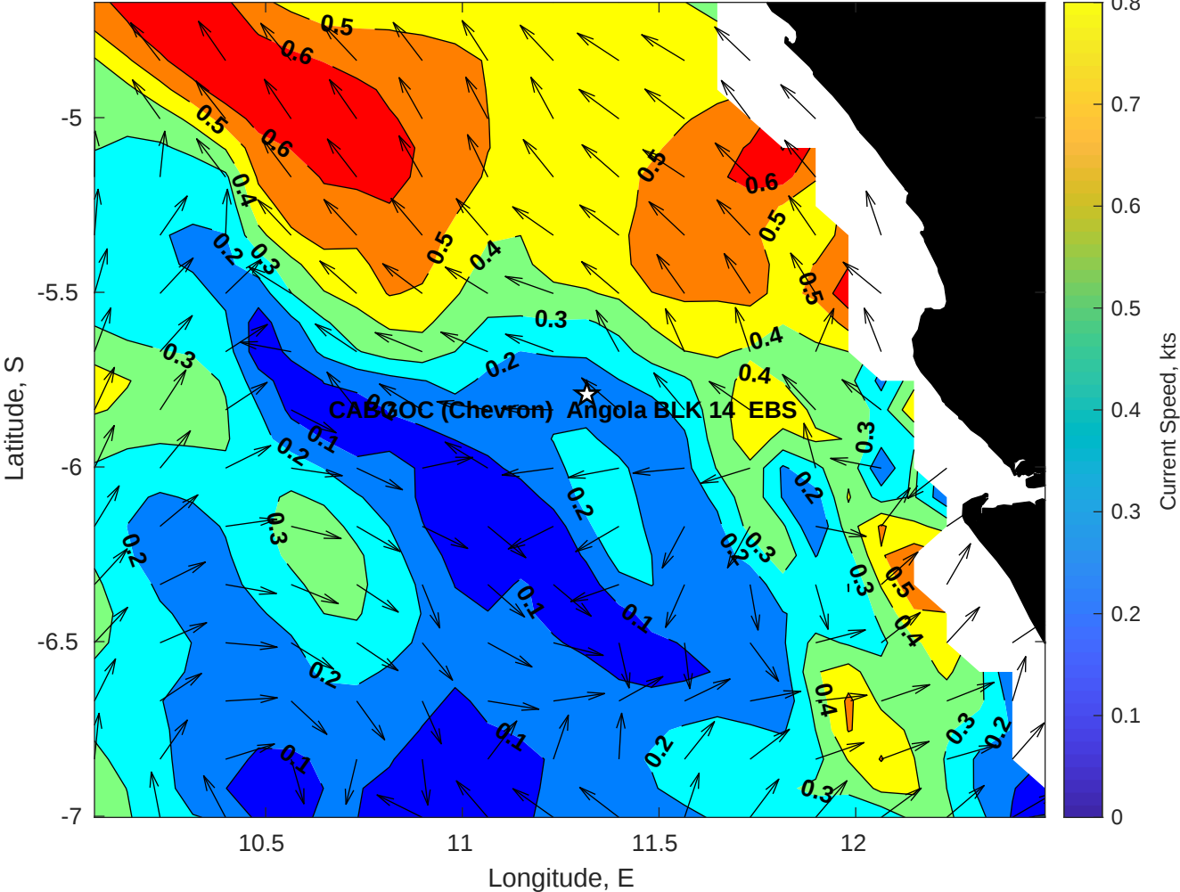
Surface Currents for CABGOC (Chevron) Angola BLK 14 EBS at 17-Apr-2025 00:00:00
