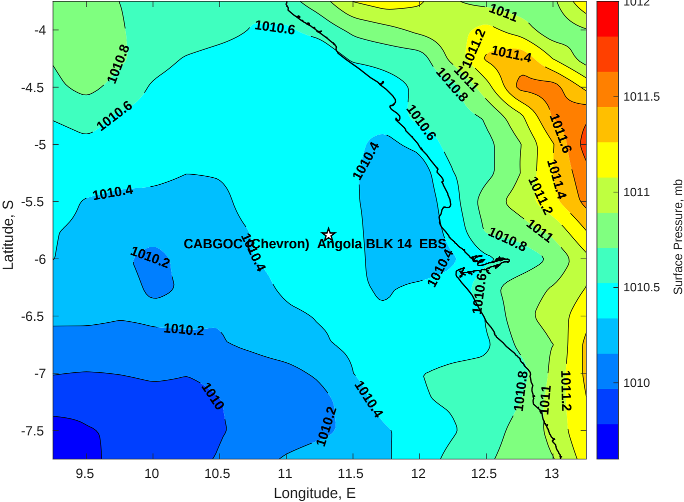
Surface Pressure (mb) for CABGOC (Chevron) Angola BLK 14 EBS at 18-Apr-2025 00:00:00
