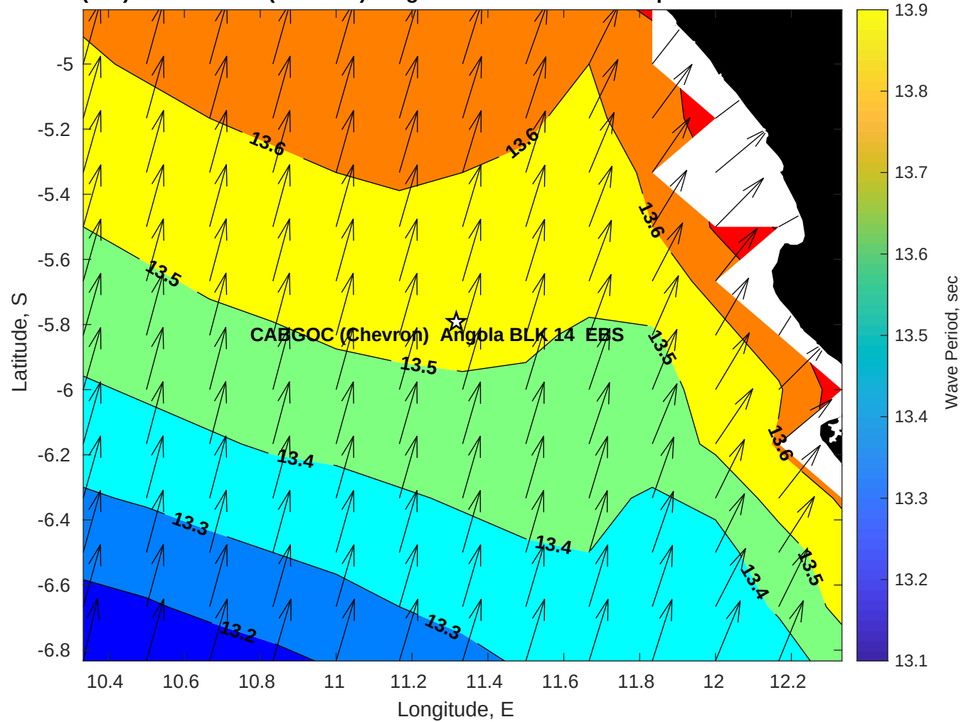
Wave Period (sec) for CABGOC (Chevron) Angola BLK 14 EBS at 18-Apr-2025 09:00:00
