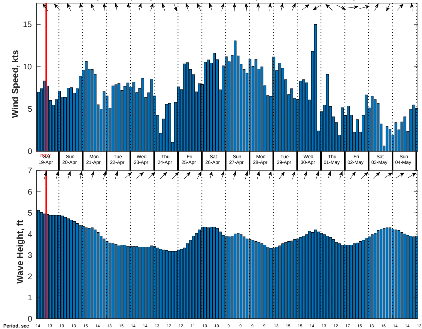
Wind & Wave Forecast for CABGOC (Chevron) Angola BLK 14 EBS from 18-Apr-2025 02:00:00 to 04-May-2025 02:00:00
