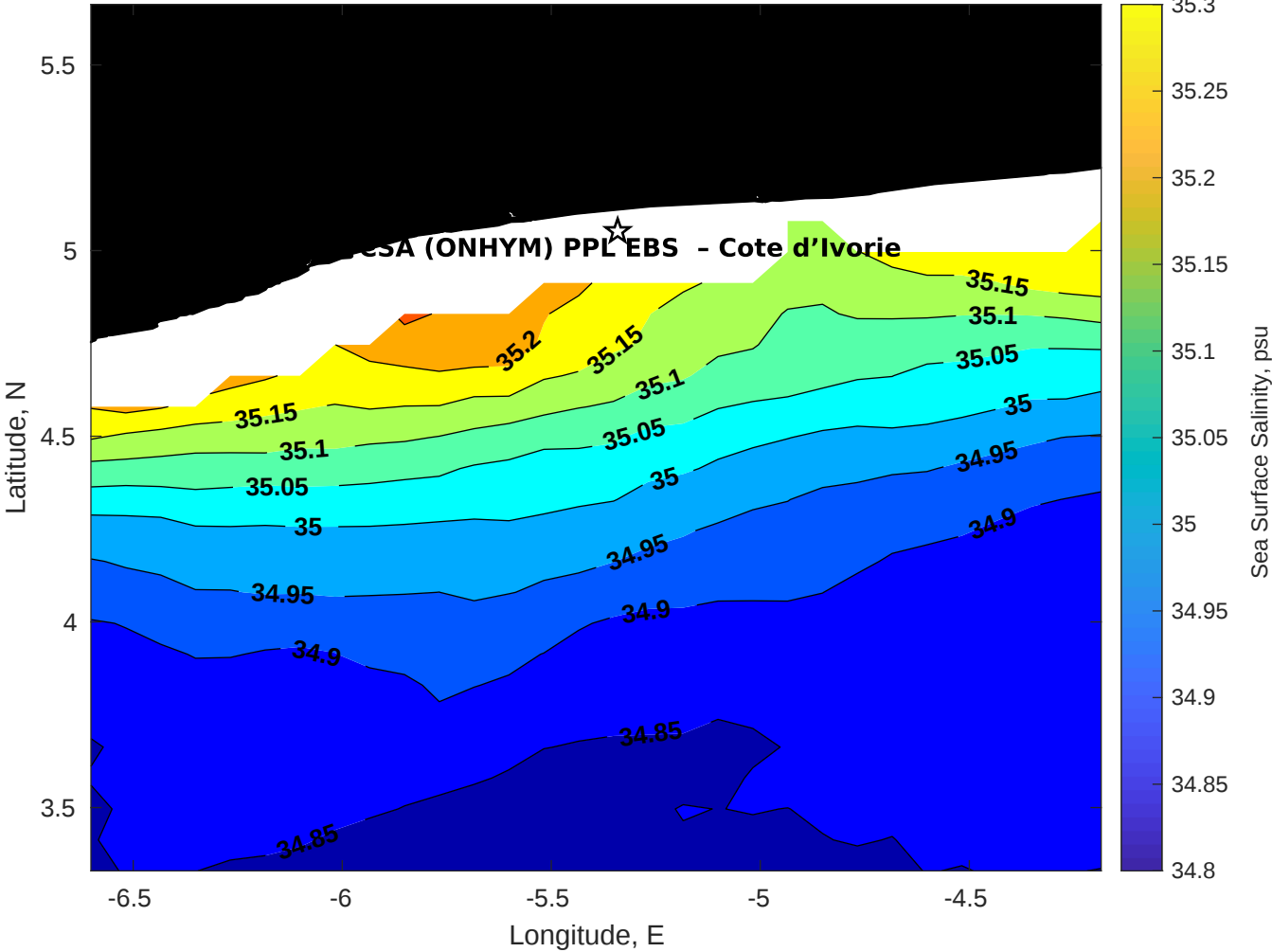
Surface Salinity for CSA (ONHYM) PPL EBS - Cote d'Ivoire at 17-Apr-2025 00:00:00
