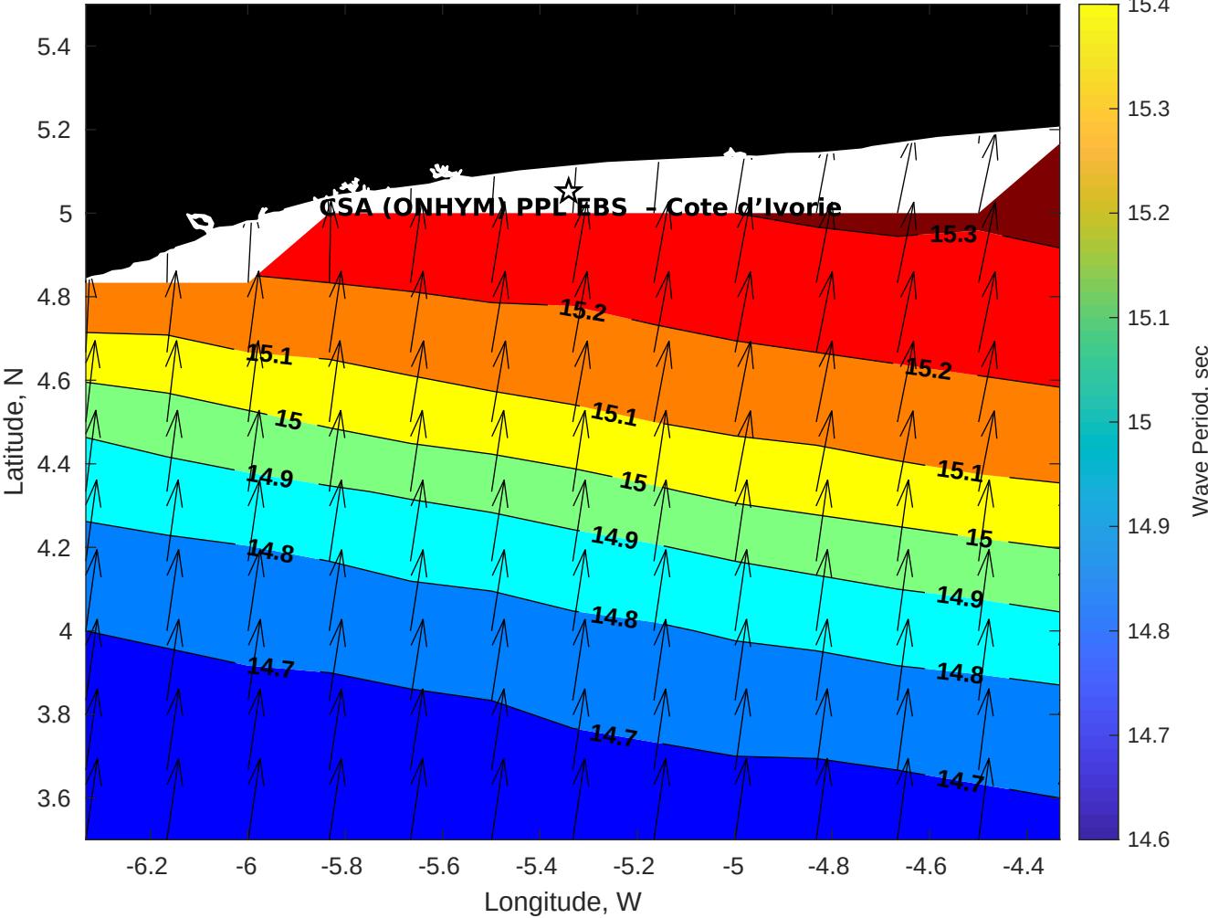
Wave Period (sec) for CSA (ONHYM) PPL EBS - Cote d'Ivoire at 18-Apr-2025 09:00:00
