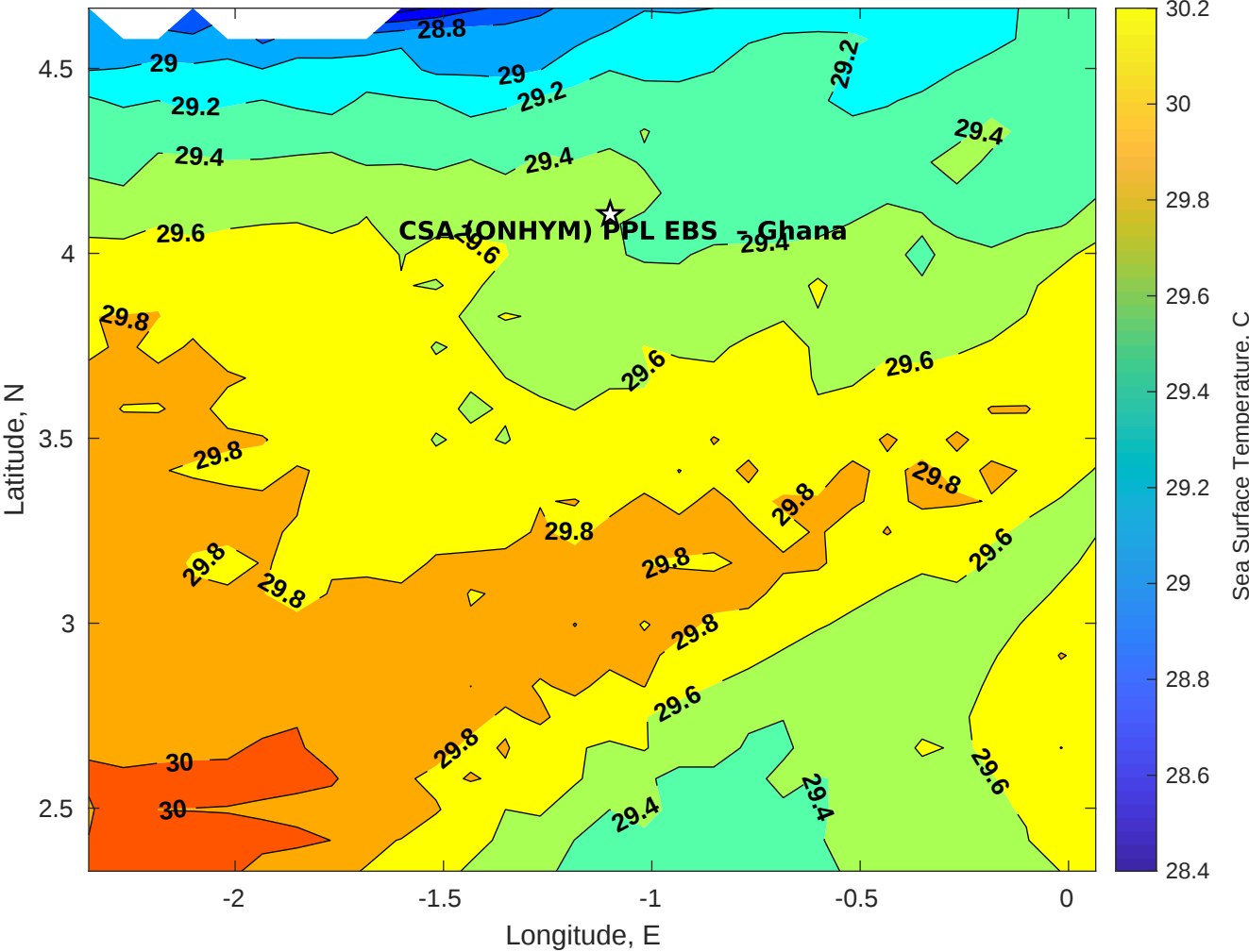
SST for CSA (ONHYM) PPL EBS - Ghana at 17-Apr-2025 00:00:00
