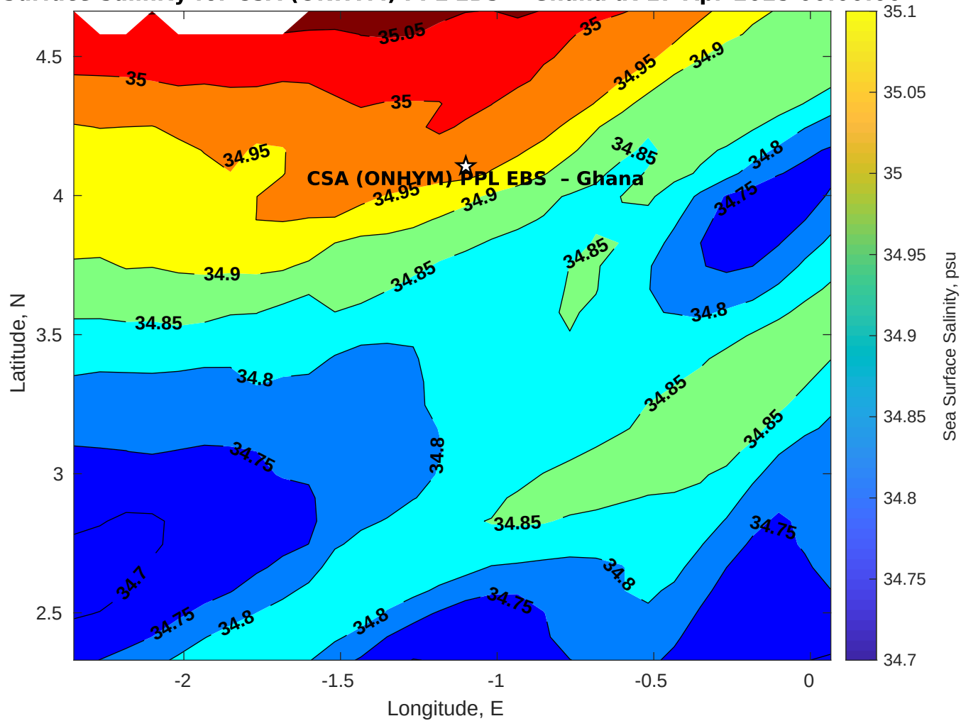
Surface Salinity for CSA (ONHYM) PPL EBS - Ghana at 17-Apr-2025 00:00:00
