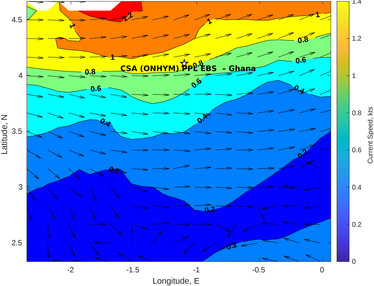
Surface Currents for CSA (ONHYM) PPL EBS - Ghana at 17-Apr-2025 00:00:00
