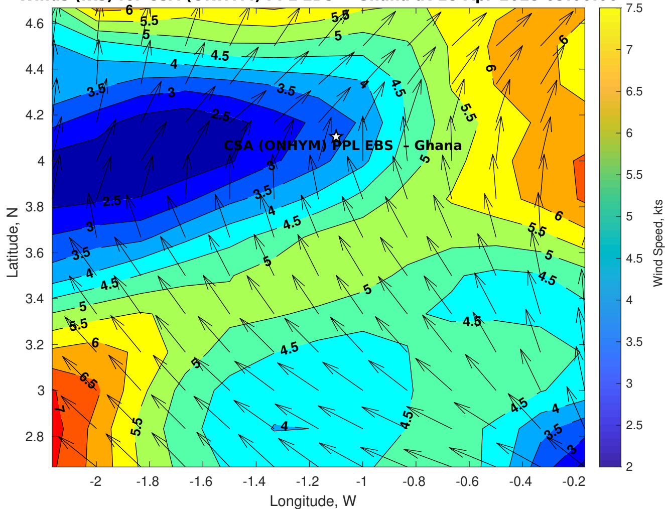
Winds (kts) for CSA (ONHYM) PPL EBS - Ghana at 18-Apr-2025 09:00:00
