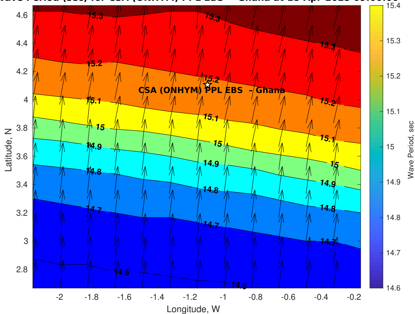
Wave Period (sec) for CSA (ONHYM) PPL EBS - Ghana at 18-Apr-2025 09:00:00
