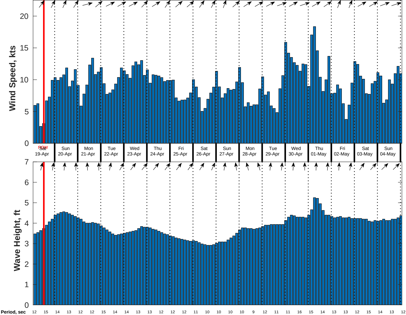
Wind & Wave Forecast for CSA (ONHYM) PPL EBS - Ghana from 18-Apr-2025 02:00:00 to 04-May-2025 02:00:00
