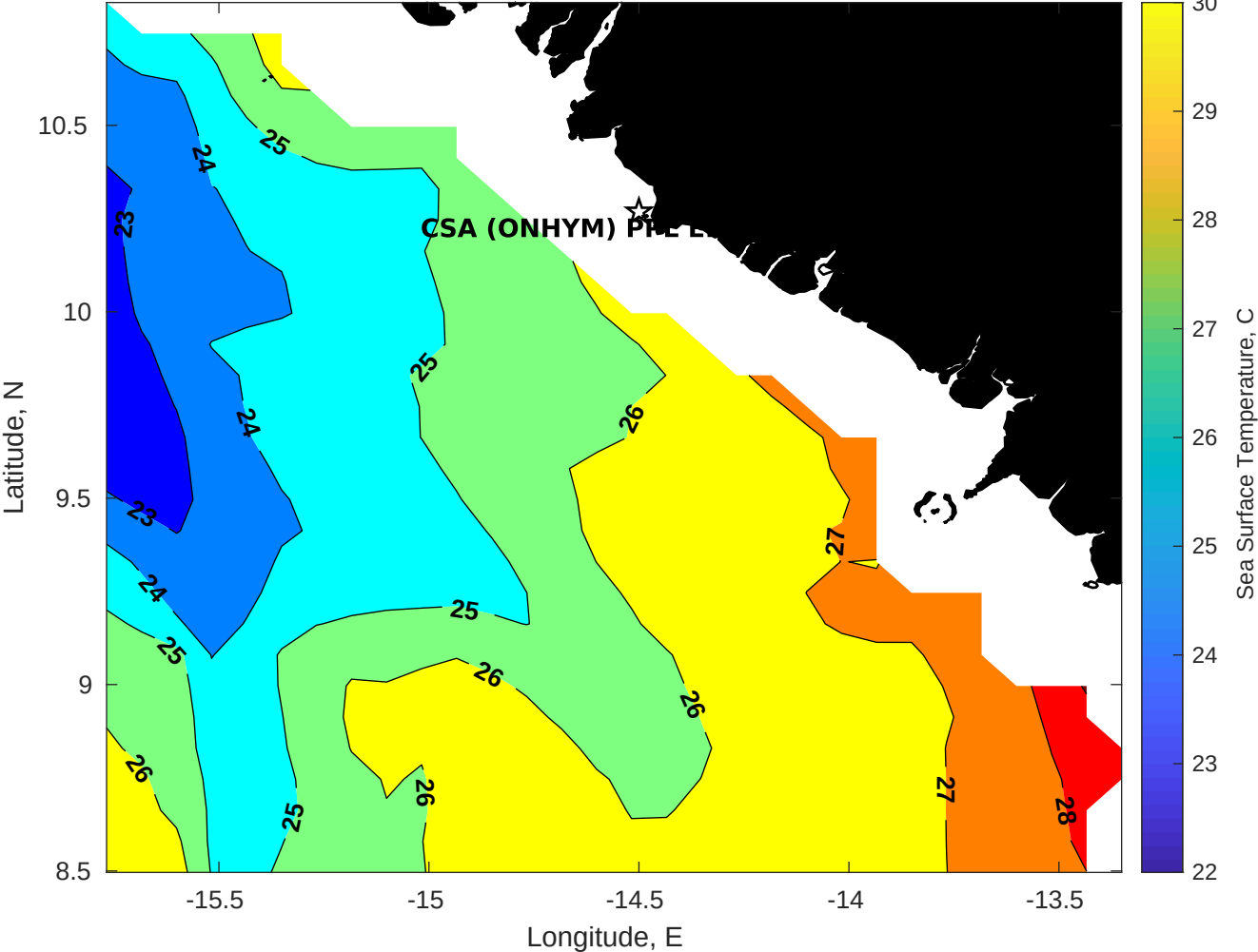
SST for CSA (ONHYM) PPL EBS - Guinea at 17-Apr-2025 00:00:00
