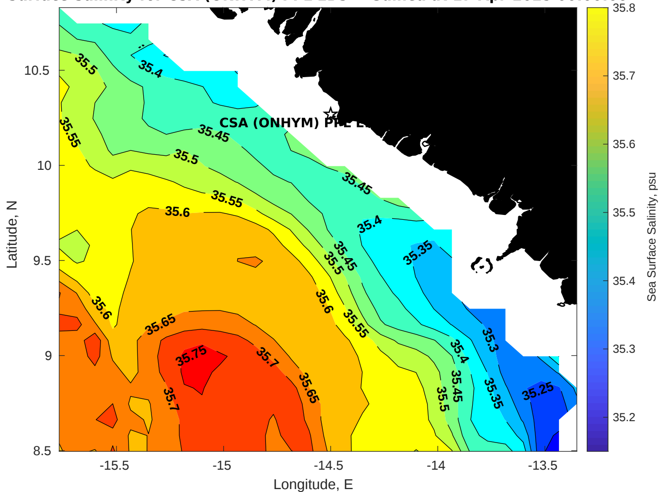
Surface Salinity for CSA (ONHYM) PPL EBS - Guinea at 17-Apr-2025 00:00:00
