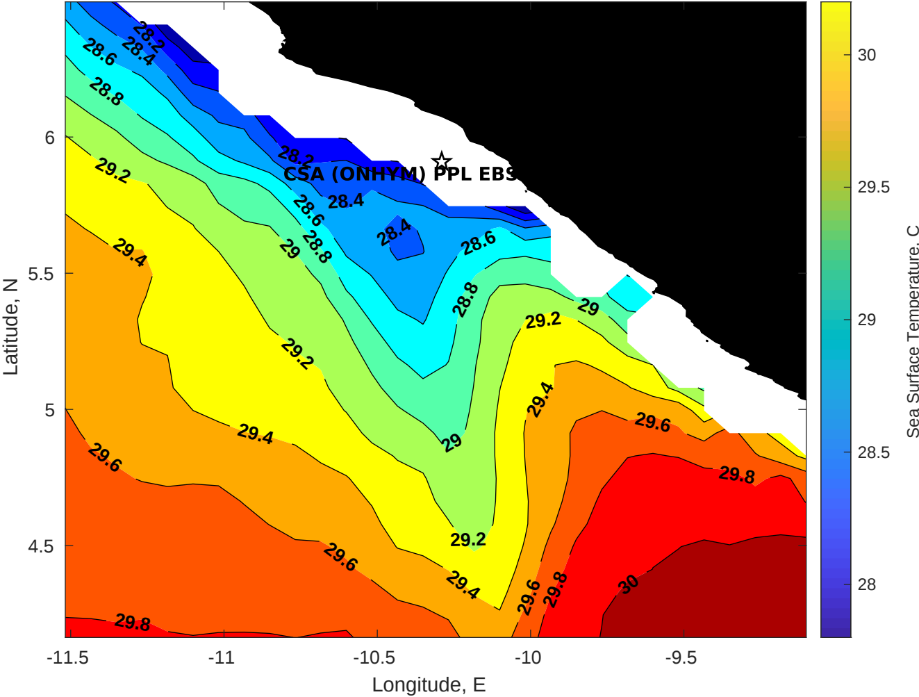
SST for CSA (ONHYM) PPL EBS - Liberia at 17-Apr-2025 00:00:00
