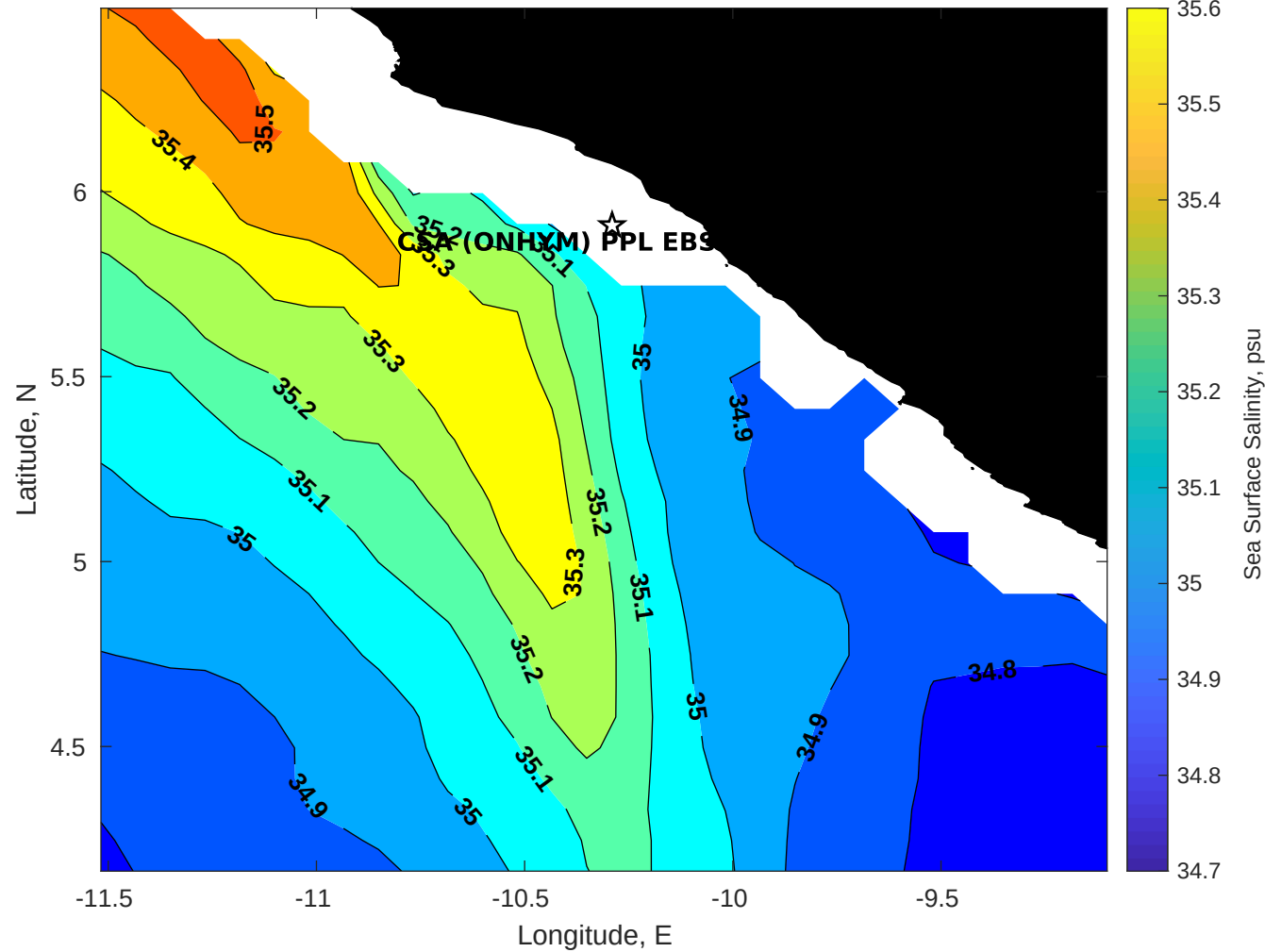
Surface Salinity for CSA (ONHYM) PPL EBS - Liberia at 17-Apr-2025 00:00:00
