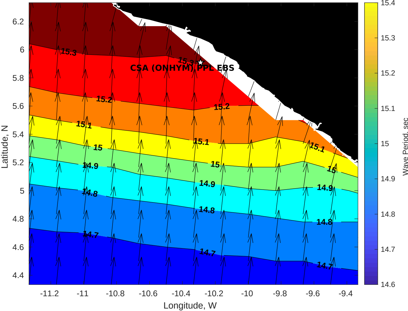
Wave Period (sec) for CSA (ONHYM) PPL EBS - Liberia at 18-Apr-2025 09:00:00
