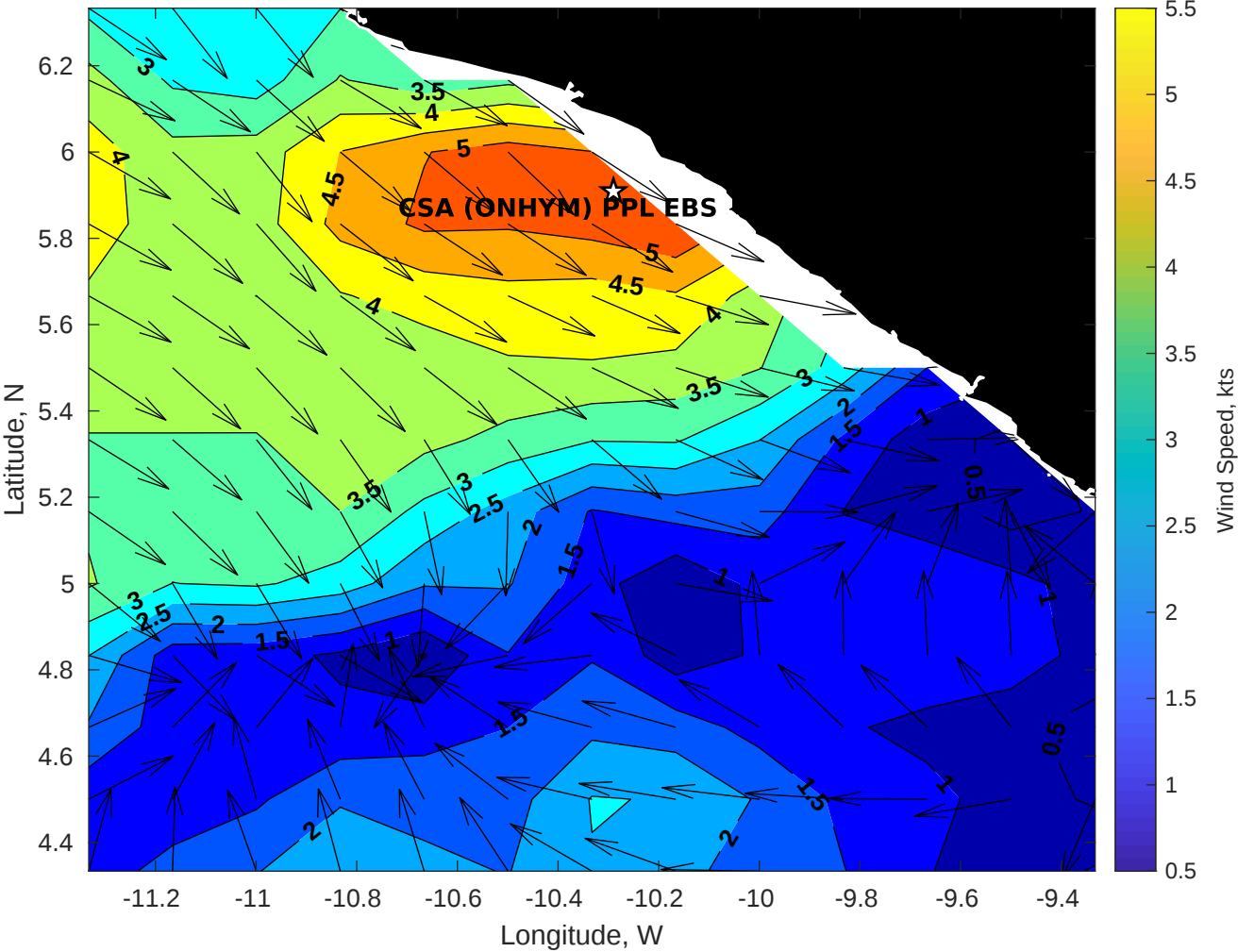
Winds (kts) for CSA (ONHYM) PPL EBS - Liberia at 18-Apr-2025 09:00:00
