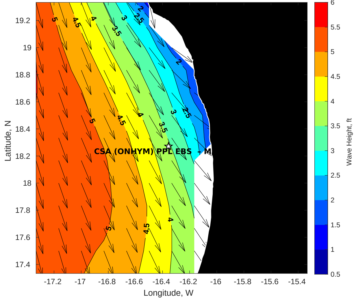
Wave Height (ft) for CSA (ONHYM) PPL EBS - Mauritania at 18-Apr-2025 09:00:00
