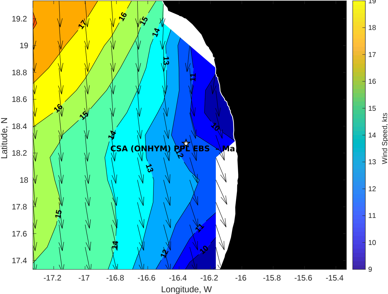
Winds (kts) for CSA (ONHYM) PPL EBS - Mauritania at 18-Apr-2025 09:00:00
