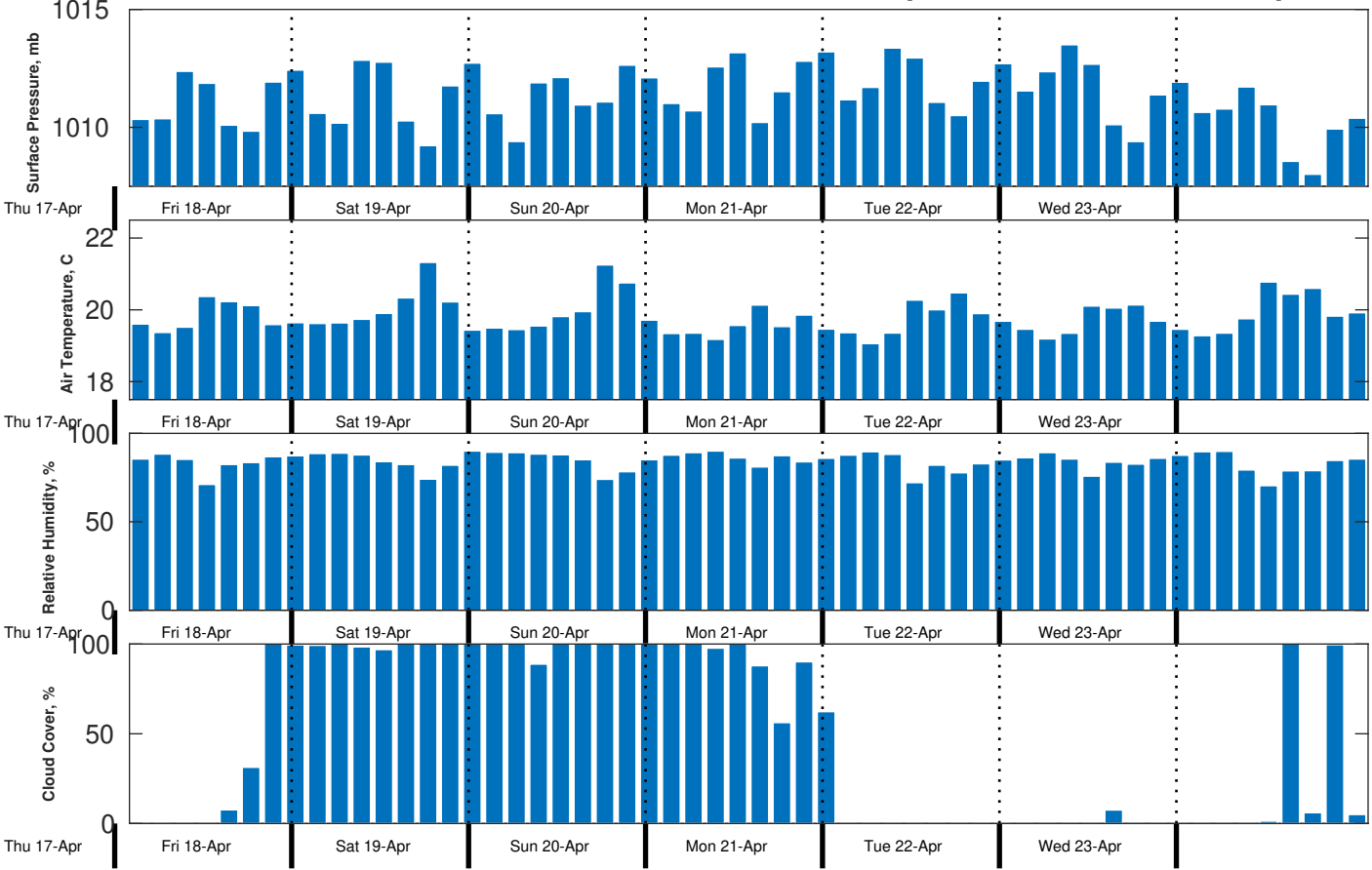
Met Forecast for CSA (ONHYM) PPL EBS - Mauritania from 18-Apr-2025 00:00:00 to 25-Apr-2025 00:00:00
