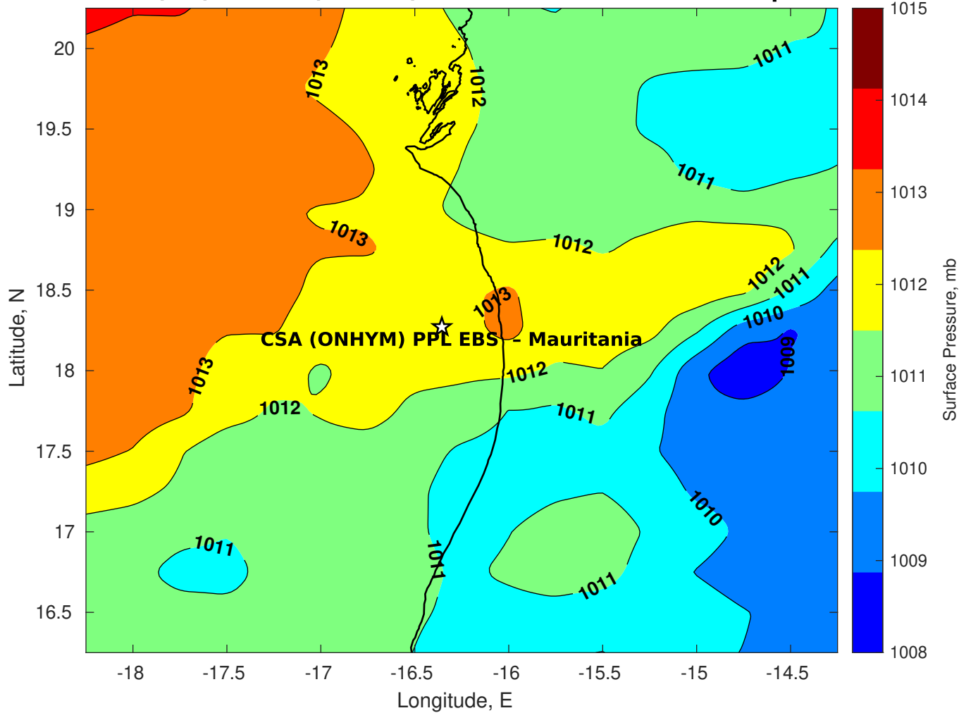
Surface Pressure (mb) for CSA (ONHYM) PPL EBS - Mauritania at 20-Apr-2025 00:00:00
