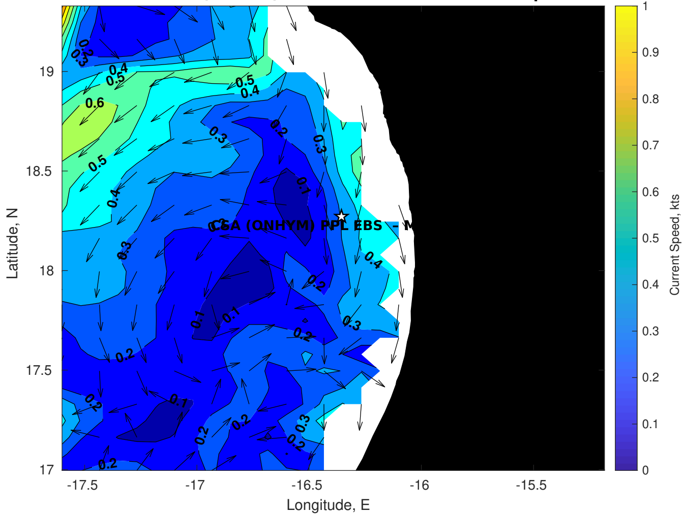
Surface Currents for CSA (ONHYM) PPL EBS - Mauritania at 17-Apr-2025 00:00:00
