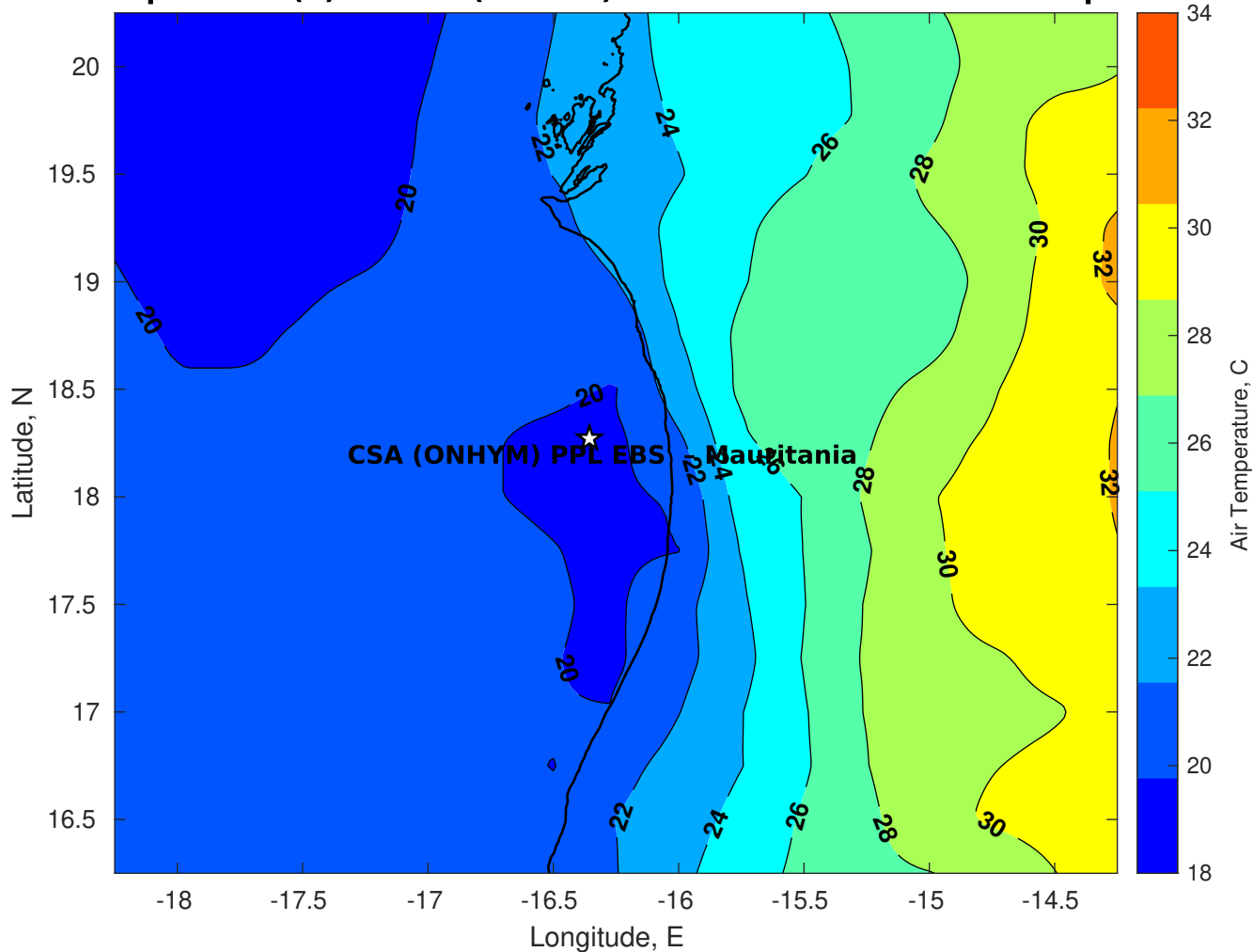
Air Temperature (C) for CSA (ONHYM) PPL EBS - Mauritania at 18-Apr-2025
