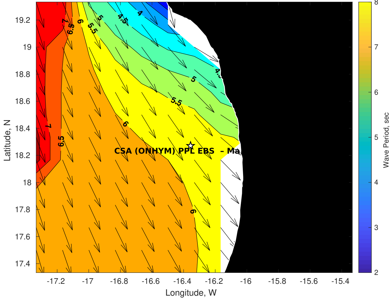
Wave Period (sec) for CSA (ONHYM) PPL EBS - Mauritania at 18-Apr-2025 09:00:00
