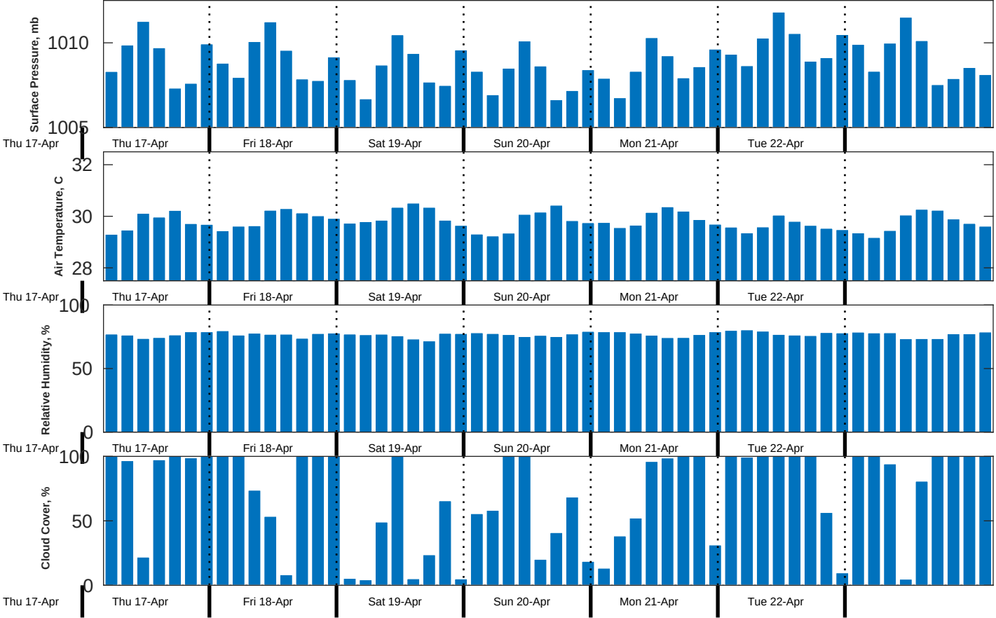
Met Forecast for CSA (ONHYM) PPL EBS - Nigeria from 18-Apr-2025 00:00:00 to 25-Apr-2025 00:00:00
