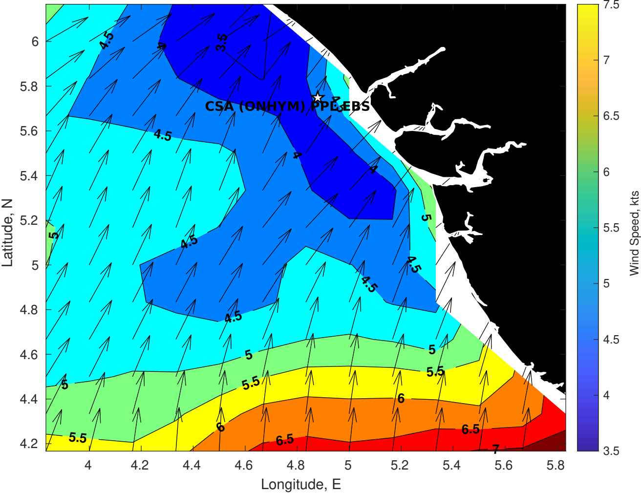
Winds (kts) for CSA (ONHYM) PPL EBS - Nigeria at 18-Apr-2025 09:00:00
