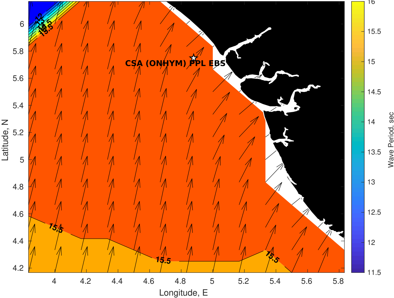
Wave Period (sec) for CSA (ONHYM) PPL EBS - Nigeria at 18-Apr-2025 09:00:00
