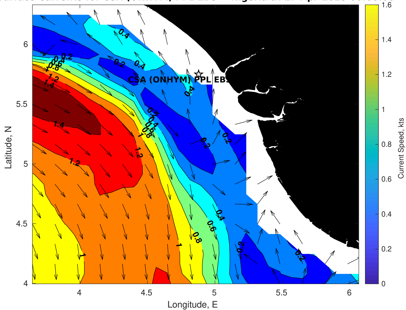
Surface Currents for CSA (ONHYM) PPL EBS - Nigeria at 17-Apr-2025 00:00:00
