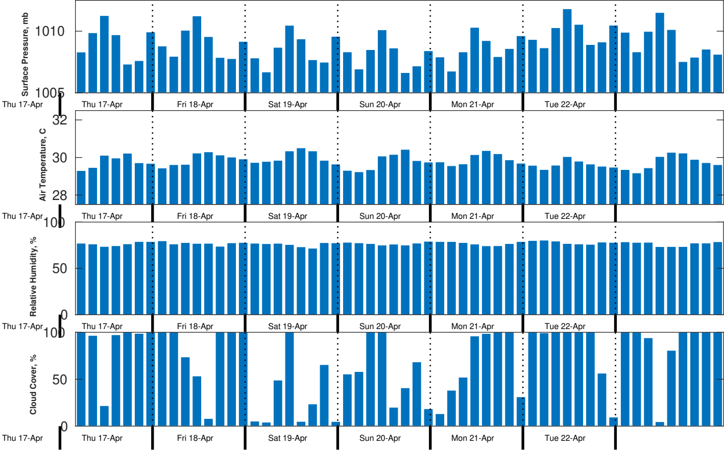
Met Forecast for CSA (ONHYM) PPL EBS - Nigeria from 18-Apr-2025 00:00:00 to 25-Apr-2025 00:00:00
