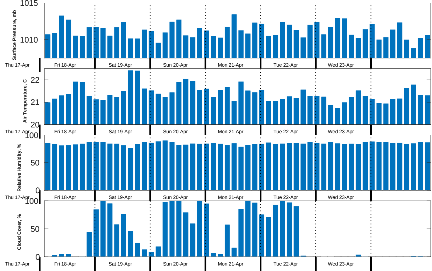
Met Forecast for CSA (ONHYM) PPL EBS - Senegal from 18-Apr-2025 00:00:00 to 25-Apr-2025 00:00:00
