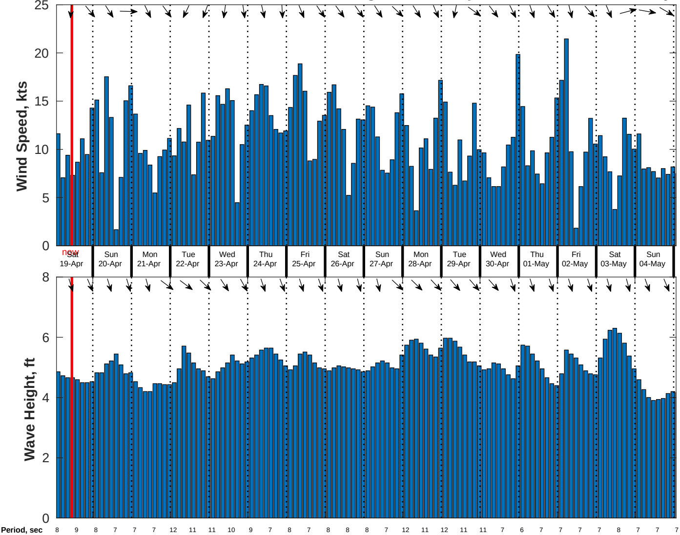
Wind & Wave Forecast for CSA (ONHYM) PPL EBS - Senegal from 18-Apr-2025 01:00:00 to 04-May-2025 01:00:00
