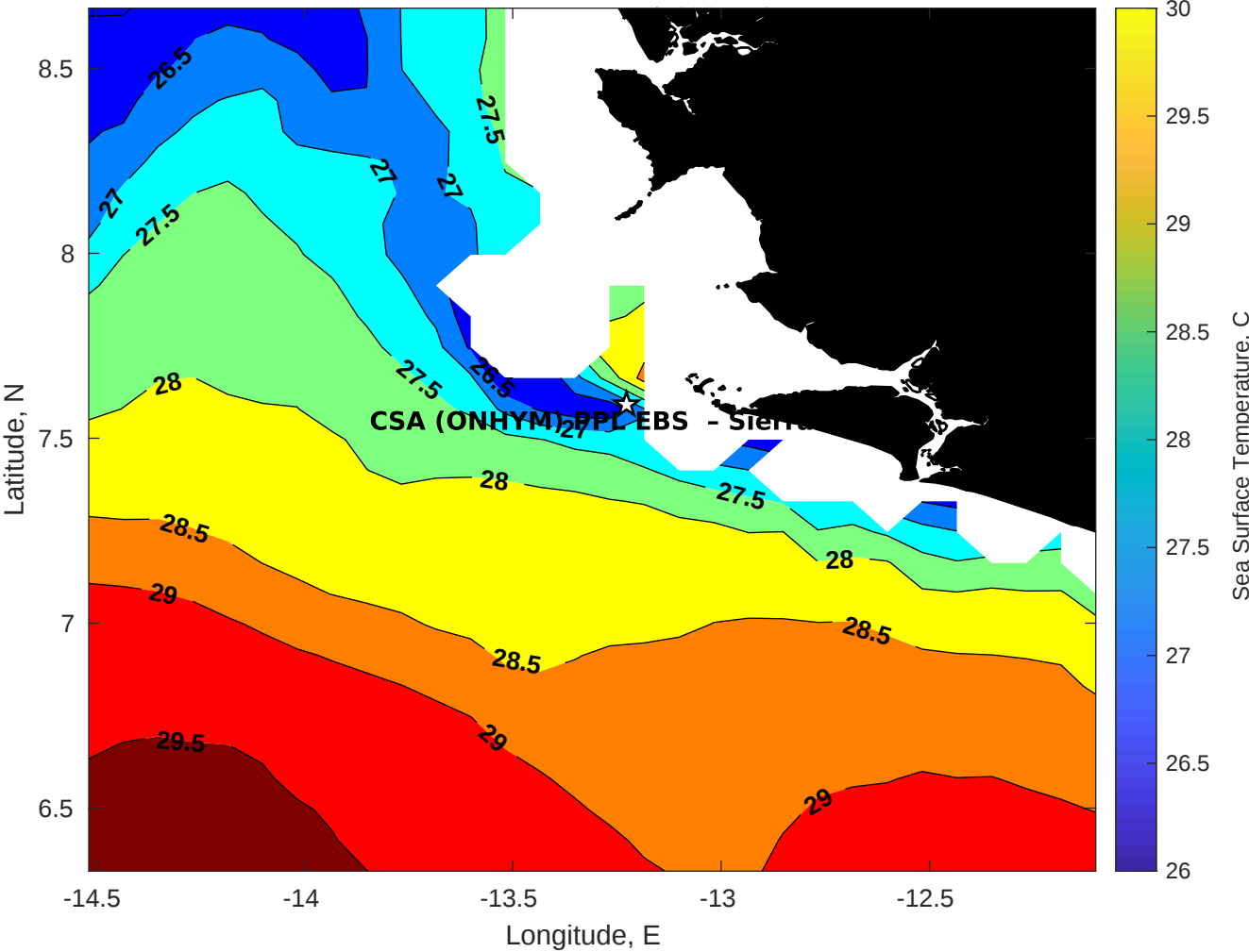
SST for CSA (ONHYM) PPL EBS - Sierra Leone at 17-Apr-2025 00:00:00
